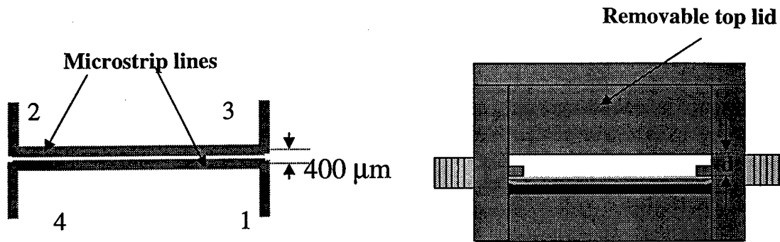
Side view of the packaged device
