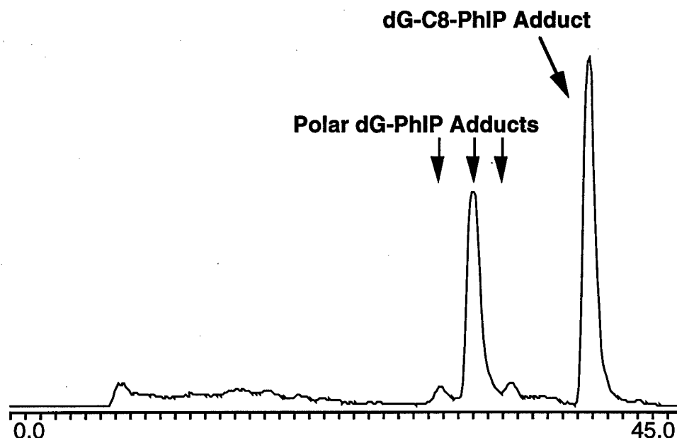
Figure 8. Typical ^{32}P -postlabeling profile for PhIP modified DNA using newly developed HPLC Inline Precolumn Postlabeling (HIPP) methods.
