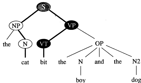
Figure 2: Parse tree from the grammar with a source path shown in white and a goal path shown in black.
