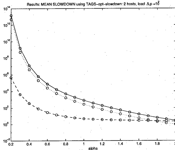
Figure 15: Mean slowdown under TAGS-opt-slowdown in a distributed server with 2 hosts with system load 0.5, as compared with the performance of Random and Least-Work-Remaining. In this set of results the task size distribution is B(k, p, \alpha) , where p = 10^7 .
