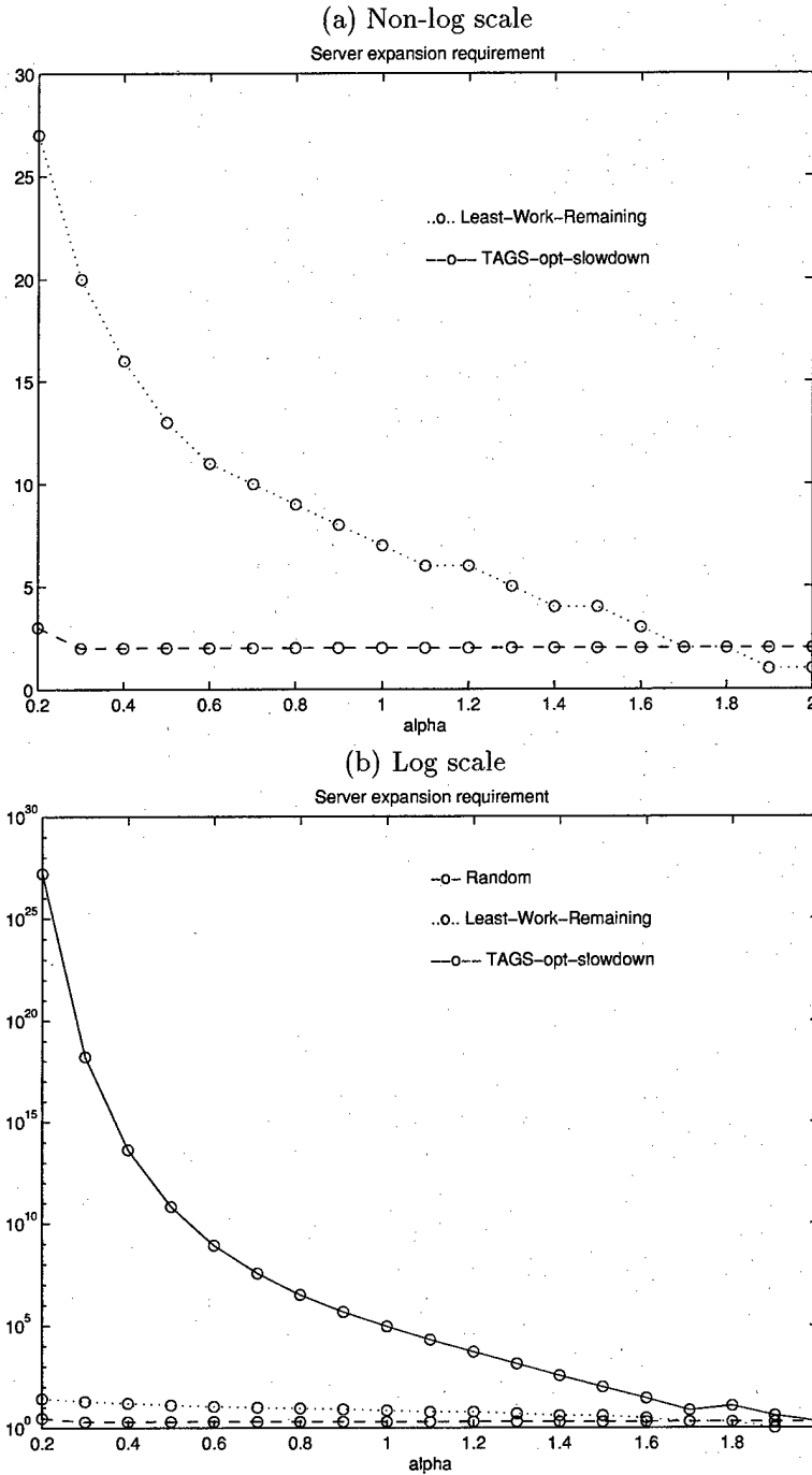
Figure 13: Server expansion requirement for each of the task assignment policies, given that we start with a 2 host system with system load of 0.7. (a) Shows just Least-Work-Remaining and TAGS-opt-slowdown on a non-log scale (b) Shows Least-Work-Remaining, TAGS-opt-slowdown, and Random on a log scale.
