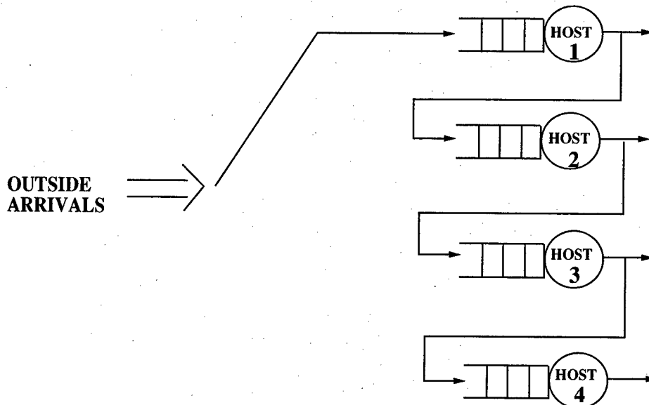
Figure 5: Illustration of the flow of tasks in the TAGS algorithm.
