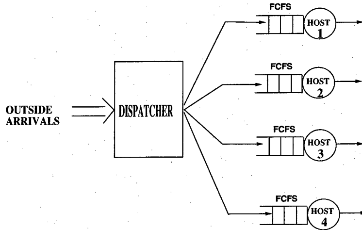
Figure 1: Illustration of a distributed server.
