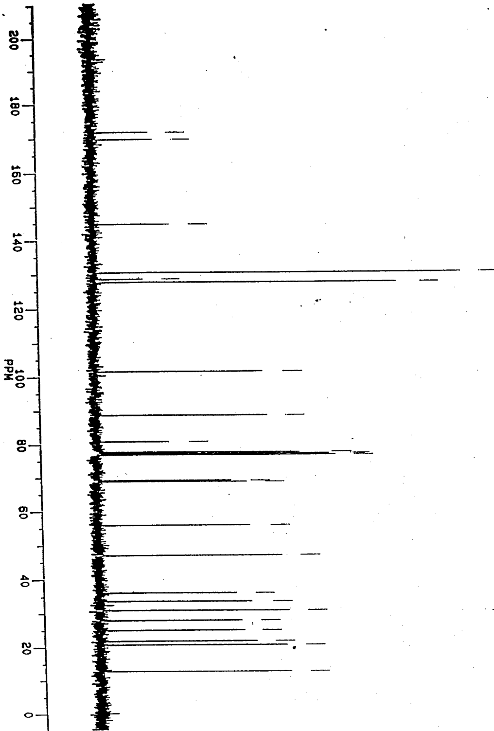
Figure 13. 13 C-nmr spectrum of rearranged artemisinic acid (R-ARTL).
