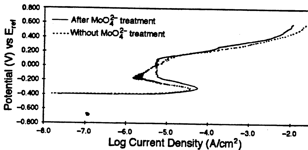
FIGURE 7. Effect of \text{MoO}_4^{2-} surface treatment on potentiodynamic polarization of type 304 SS in deaerated 0.1 M HCl ( E_{\text{ref}} = E_{\text{SCE}} ).
