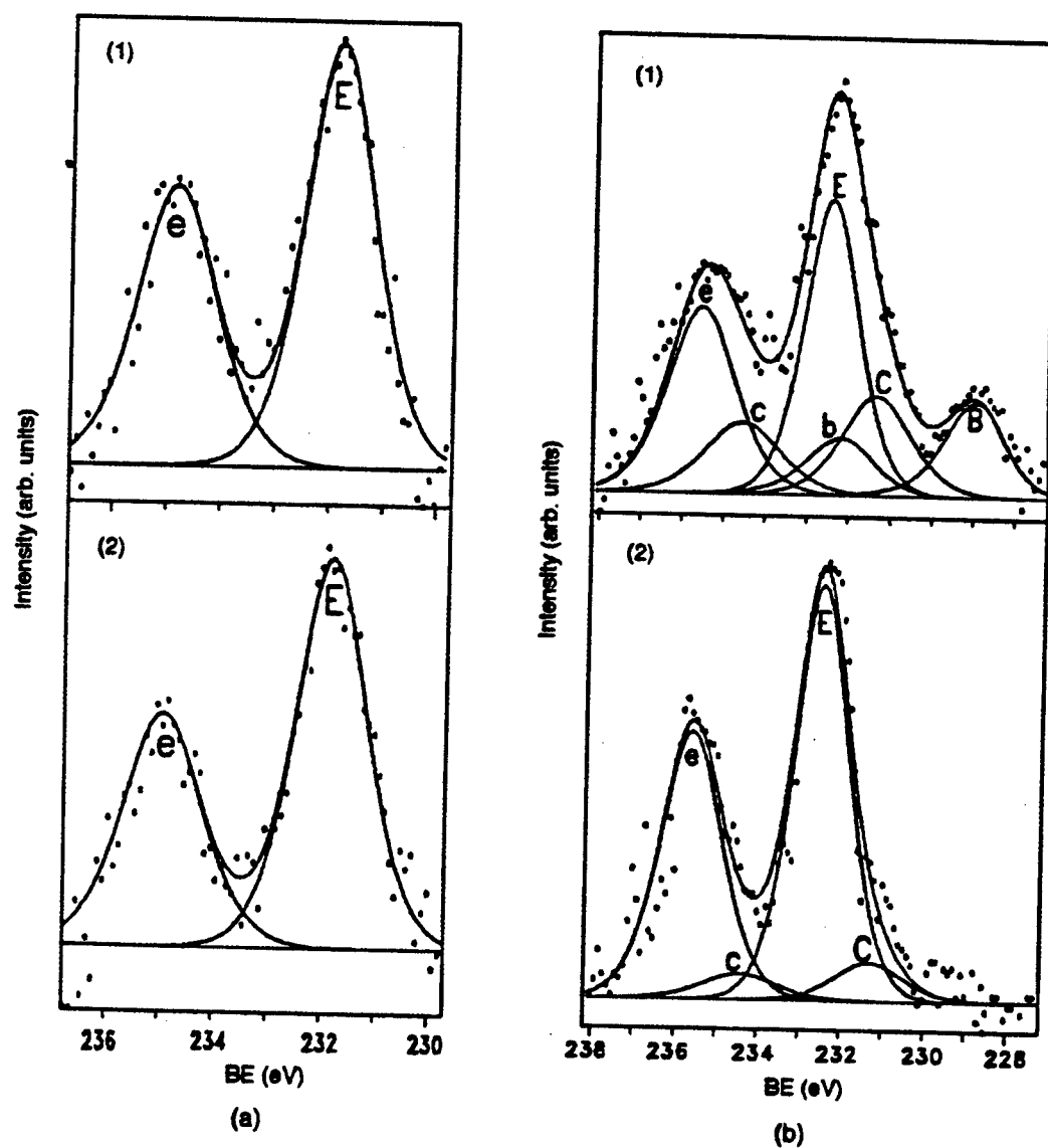
FIGURE 4. Influence of the deaerated protein-containing exopolymer of D. marina on Mo3d on the surface of type 304 SS (a) before exposure and (b) after exposure following MoO 4 2- treatment at: (1) takeoff angle of 20° and (2) takeoff angle of 50° (B, b: MoO 2 ; C, c: Mo 5+ ; and E, e: MoO 4 2- ).
