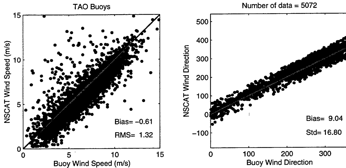
Figure 23: Scatterplots of wind speeds (left) and directions (right) comparing TAO winds with NSCAT 25 km high resolution data for angles differing by 90° or less (top) and by 60° or less (bottom). Overall bias and RMS values in lower right of each panel. There were 5253 co-locations within 90° and 5072 co-locations within 60°.
