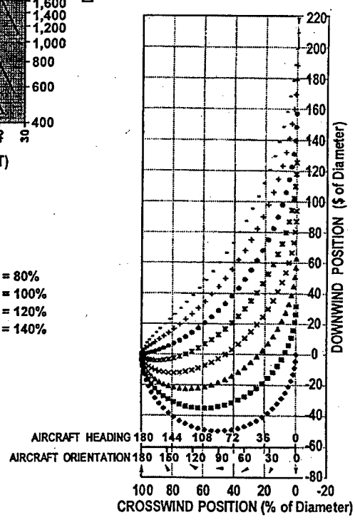
Figure 6E CONSTANT END POSITION RIGHT TURN UPWIND
