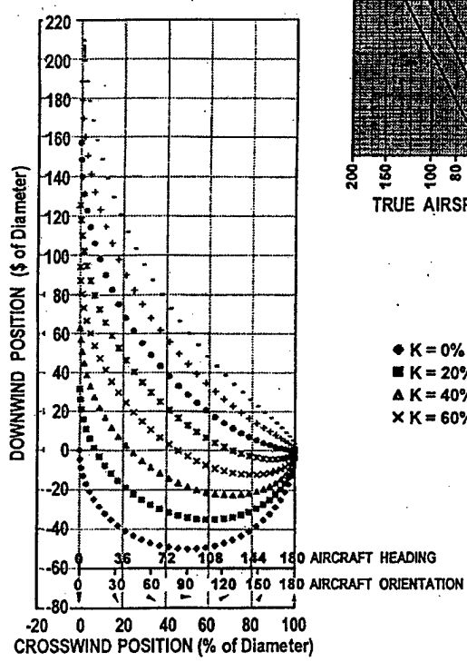
Figure 6D CONSTANT END POSITION LEFT TURN UPWIND
