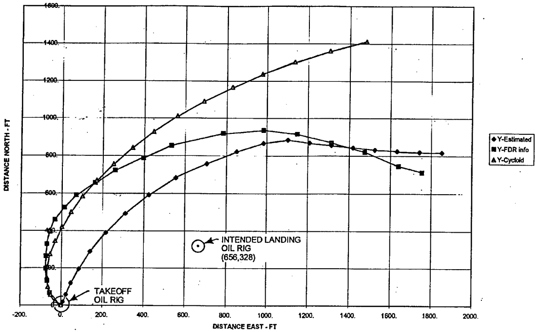
Figure 3 ESTIMATE, FLIGHT DATA RECORDER, AND CYCLOID COMPARISON
