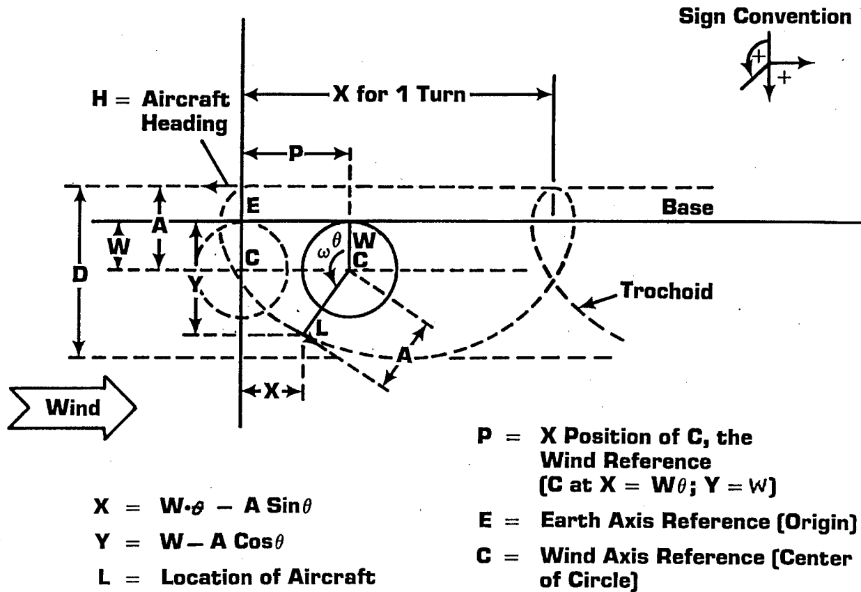
Figure 1 CYCLOID FLIGHT PATH DEFINITION
