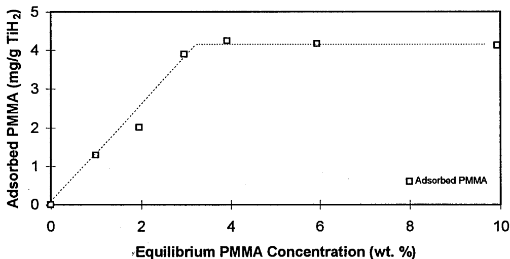
Figure 1 Adsorption isotherm for PMMA on TiH 2 powder in acetone.
