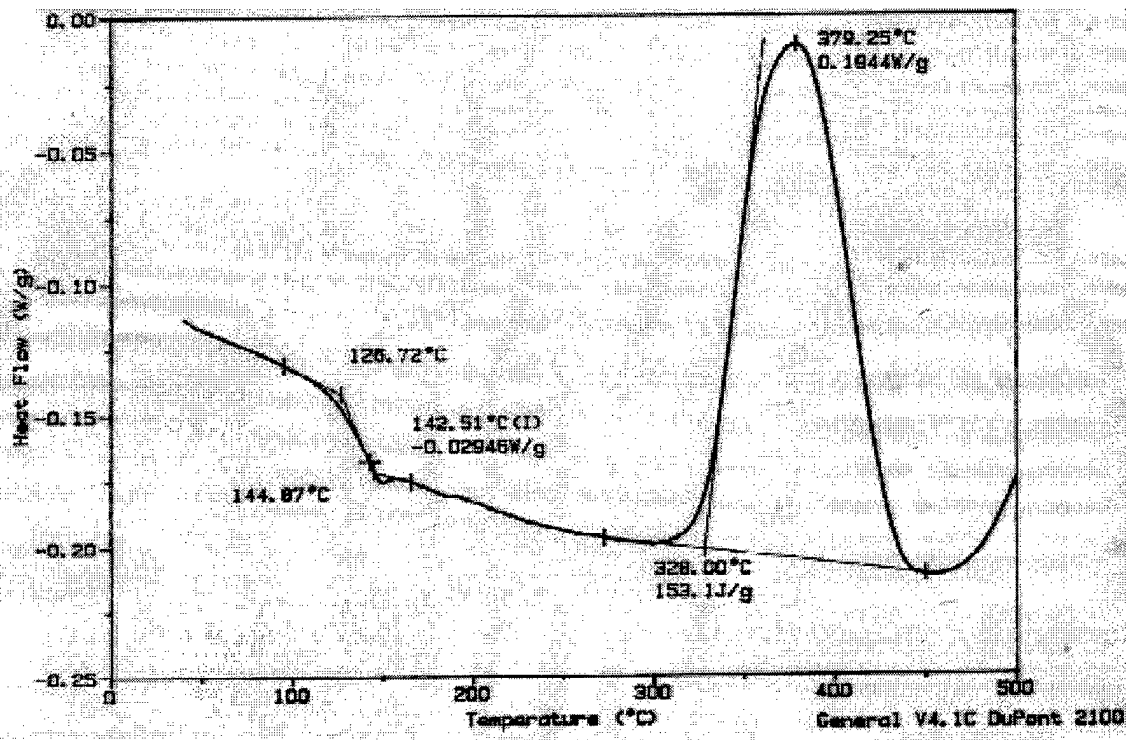
Figure 1. DSC curve of uncured PETI-RFI at 5°C/min.
