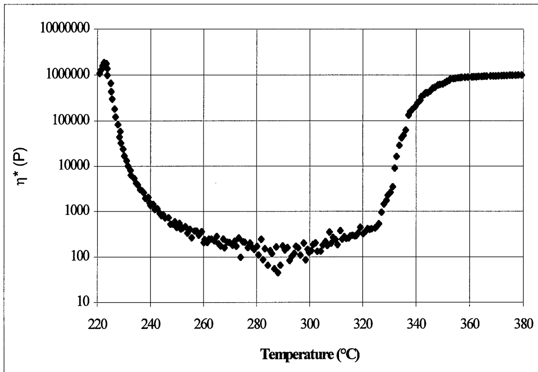
Figure 8. Complex viscosity of PETI-RFI during heating at 5^{\circ}\text{C}/\text{min} .
