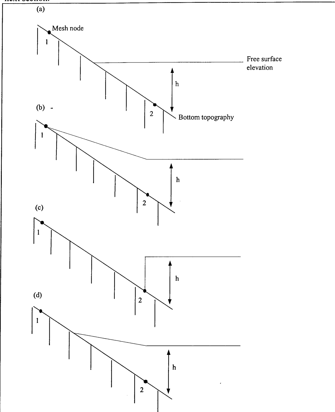
Figure 3-3 Partially dry elements: (a) the real situation, (b) element remaining fully wet introducing spurious momentum terms, (c) element exclusion method and (d) TELEMAC-2D method keeping the element partially dry (after Price, 1997).
