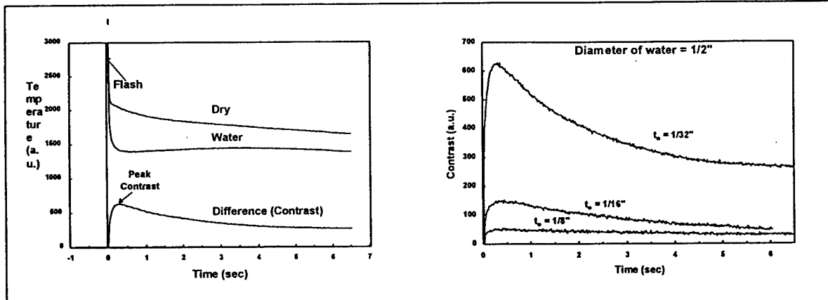
Fig. 2: (Left) This fig. shows the data curves require to generate a single contrast curve. The curve labeled "Water" represents the thermal time history of a point on the surface of the aluminum panel directly beneath a straw with filled with water. The curve labeled "Dry" represents the thermal time history of a point away from any water. The contrast curve was generated by subtracting the previous two curves. (Right) This figure shows three contrast curves for three identical water drops but for three different aluminum plate thickness.
