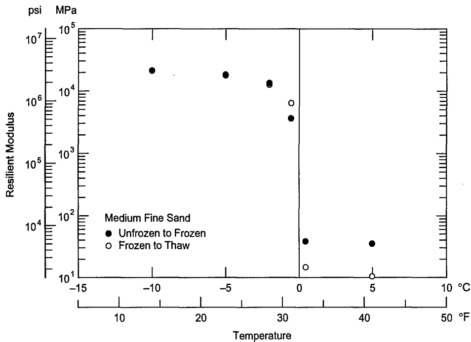
Figure 7. Effect of freezing and thawing on the resilient modulus of fine sand.
