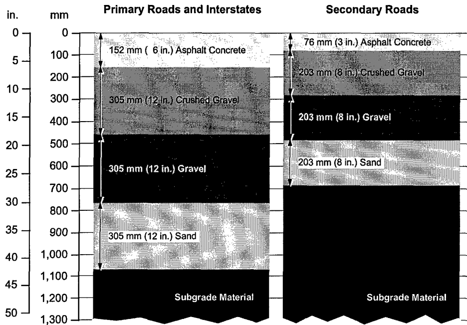
Figure 10. Typical pavement cross sections used by NHDOT.
