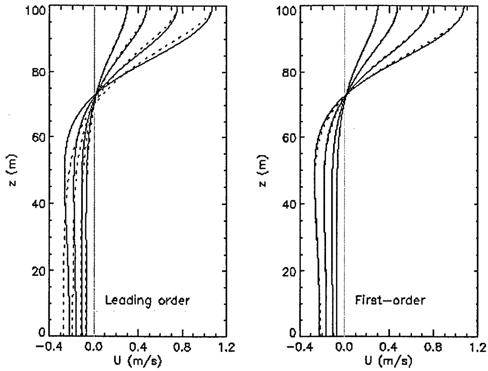
Figure 3. Horizontal velocity profiles. Density 1. Comparison of leading- and first-order Eulerian approximations (dashed) with fully nonlinear waves (solid).
