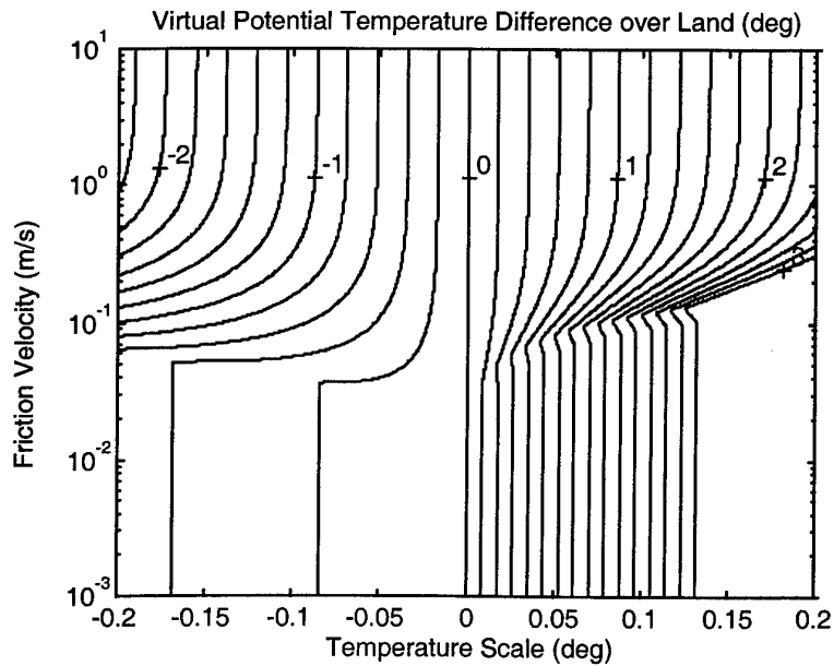
Figure 9: Contour plots showing the dependence over land of (a) wind speed and (b) virtual potential temperature difference at a height of 10 metres on friction velocity ( u_* ) and temperature scale ( \theta_* ), when the surface layer height has been taken into account.
