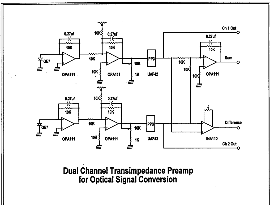
Figure 7 Circuit of the Optical Receiver and Analog Signal Processing Elements
