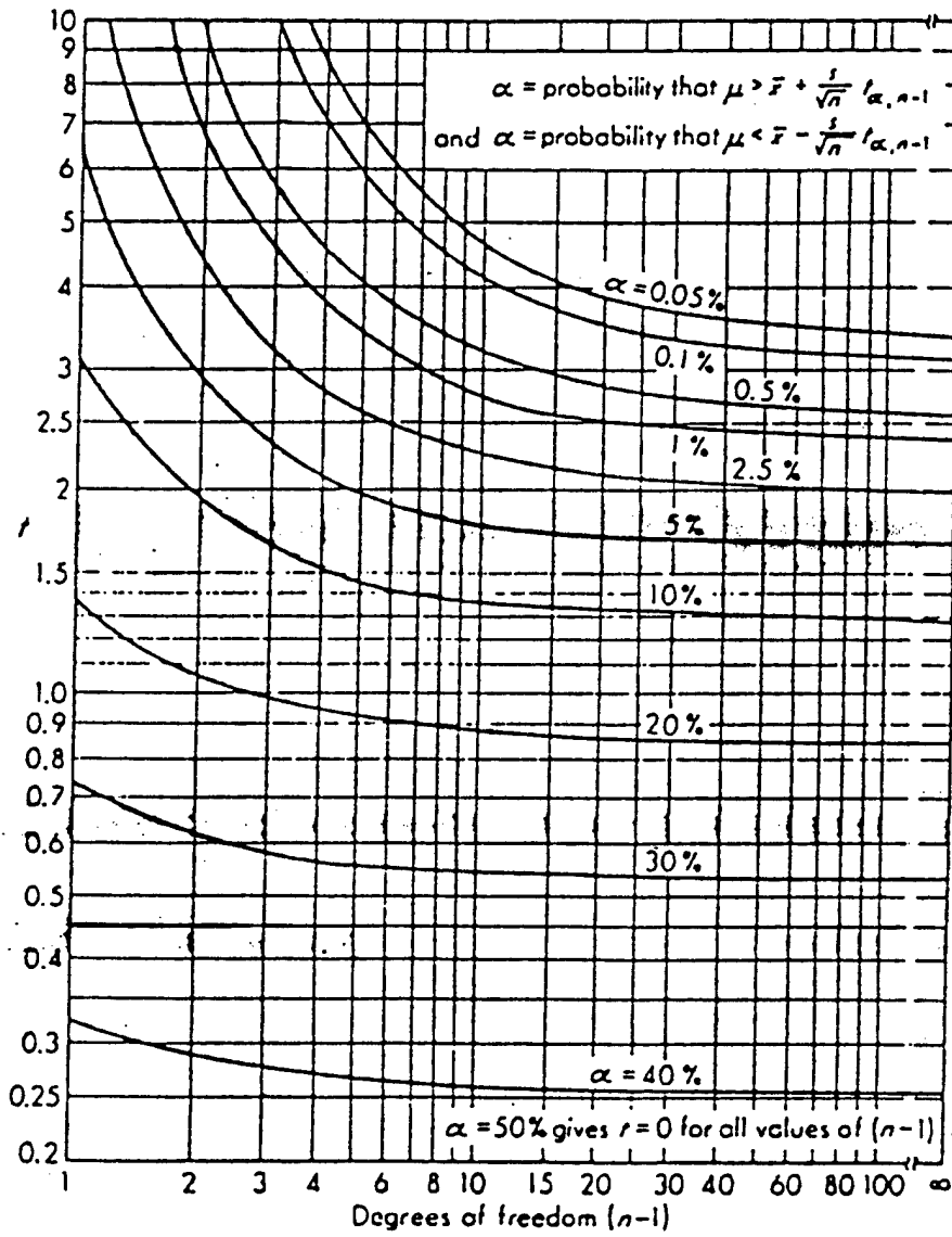
Figure 2 Student's t-function
