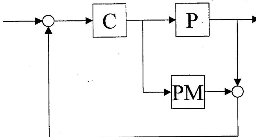
Figure 1.5 Internal-Model Control Structure
