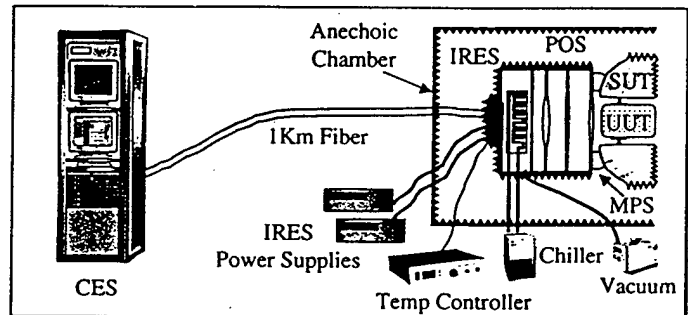
Figure 4-1. Conceptual Chamber Configuration
