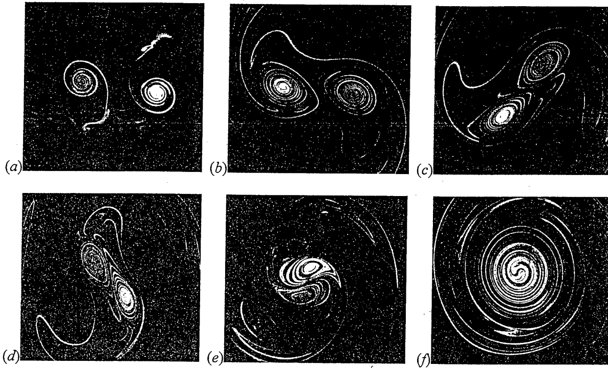
Figure 1 - Visualisation of the merging of two co-rotating vortices at Re \approx 5000 . (a) t^* = 0 , (b) t^* = 0.5 , (c) t^* = 0.6 , (d) t^* = 0.7 , (e) t^* = 0.9 , (f) t^* = 2 . t^* = t I 72 \pi^2 b^2 .
