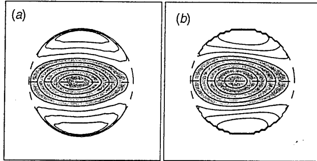
Figure 2: Comparison between the numerical (a) and analytical (b) vertical vorticity of the zigzag eigenmode in the horizontal plane for F_h = 0.033 , k_z = 8.25 , Re = 10000 .
