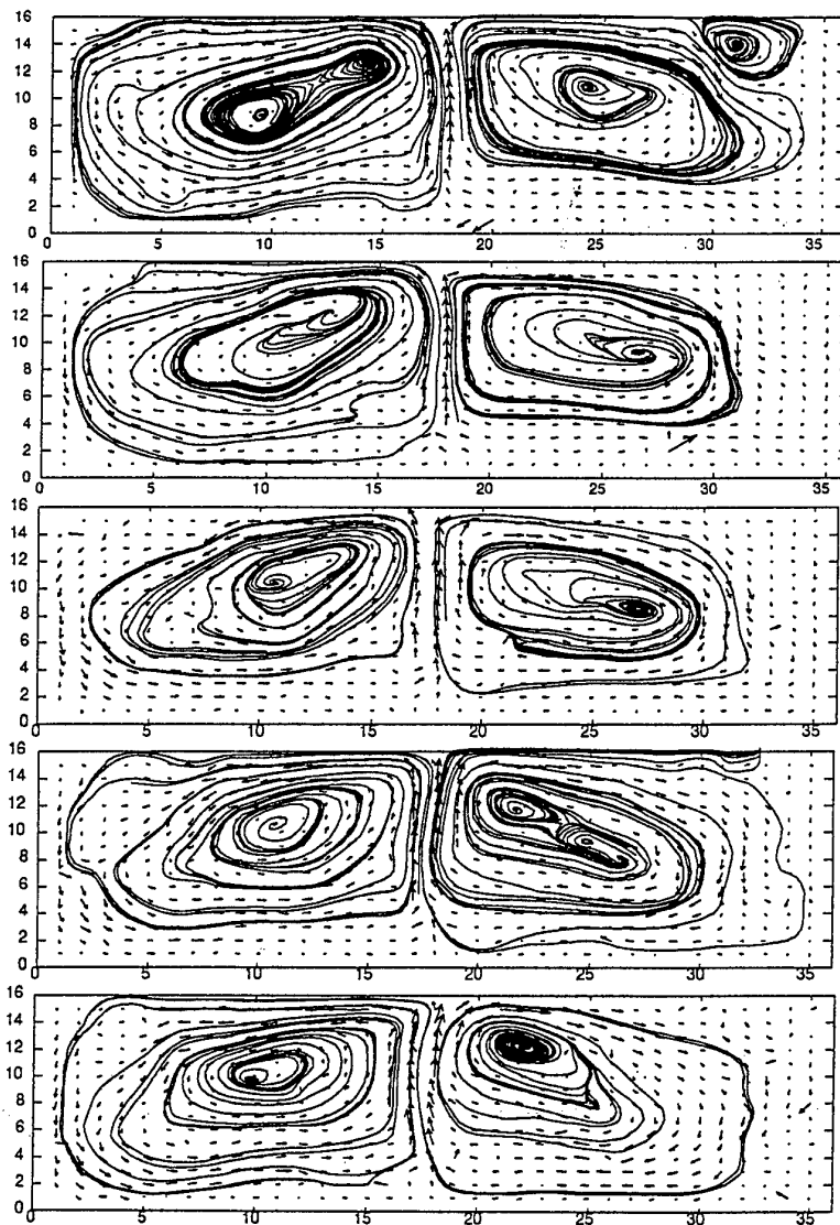
Fig. 1 Instantaneous velocity fields during a complete oscillation of the plume
