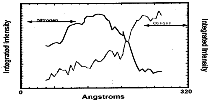
Figure 2(b). EELS Integrated Intensity for Oxygen and Nitrogen
