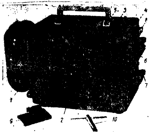
Fig. 5. Six-channel PO-6M oscill- ograph with autonomous electric feeding; 1 --tape cassette; 2--door of the body; 3--filament resistor; 4-- illuminator 5--marker breaker; 6--terminals for connecting the pickups; 7--terminals for connec- ting the marker; 8--ears for sus- pending the instrument on shock absorbers; 9--frame with dull screen for setting the optics; 10--starting switch.
