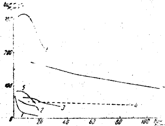
Fig. 5. Specific energy per unit volume as a function of the specific power for different electrochemical sources of current: 1--manganese-zinc batteries; 2--cadmium-nickel storage batteries; 3--lead-acid storage batteries; 4--nonlamellar cadmium-nickel storage batteries; 5--copper-magnesium cells; 6--mercury oxide cells; 7--silver-zinc storage batteries.
