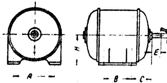
Installation dimensions of A2 and A02 electric motors
