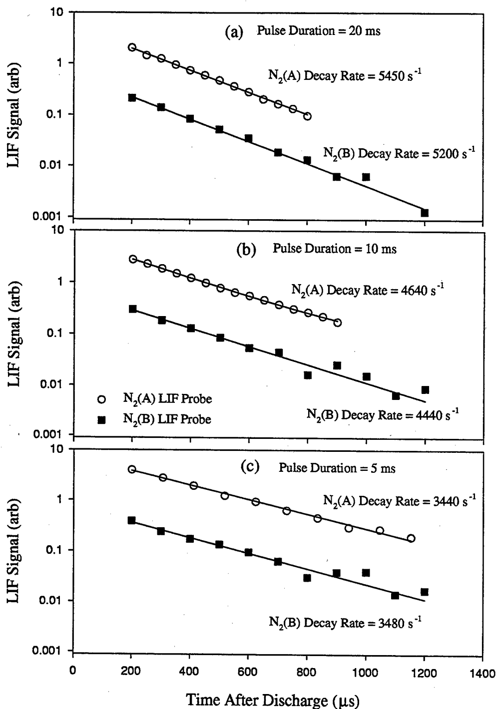
Figure 24: Comparison of \text{N}_2(\text{A}) and \text{N}_2(\text{B}) temporal decay rates at pulse durations of (a) 20 ms, (b) 10 ms, and (c) 5 ms where the similarity in \text{N}_2(\text{A}) and \text{N}_2(\text{B}) decays indicate that [\text{N}_2(\text{A})] \ll [\text{N}_2(\text{X}, v \geq 5)] in each case
