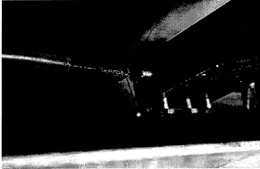
Figure 29. Flexible Hose with Custom Four-Jet Nozzle Entering Actual Jet Engine Tube Section
