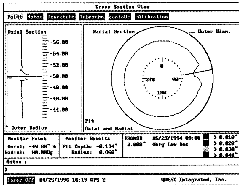
Figure 24. Cross-Sectional View of Tube with ID Scale
