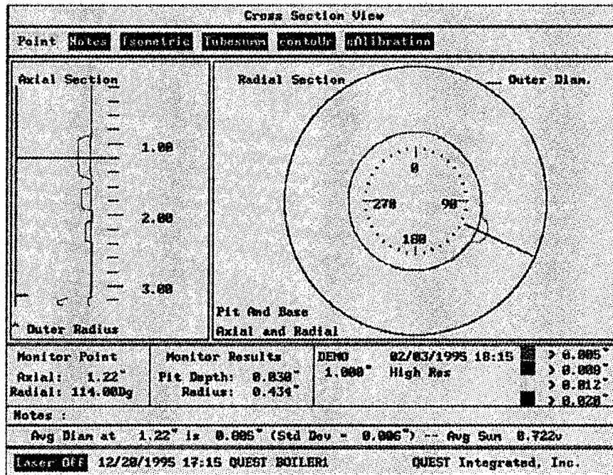
Figure 21. Cross-Sectional View
