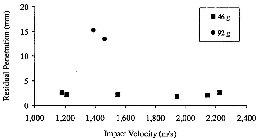
Figure 16. Residual Penetration as a Function of Impact Velocity.
