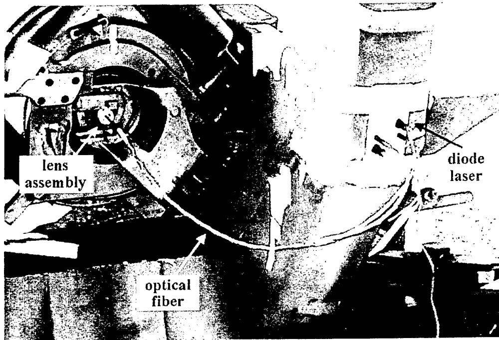
Figure 3. Diode Laser and Optical Fiber Cable to Breech During October 1998 Study With M198 Howitzer.
