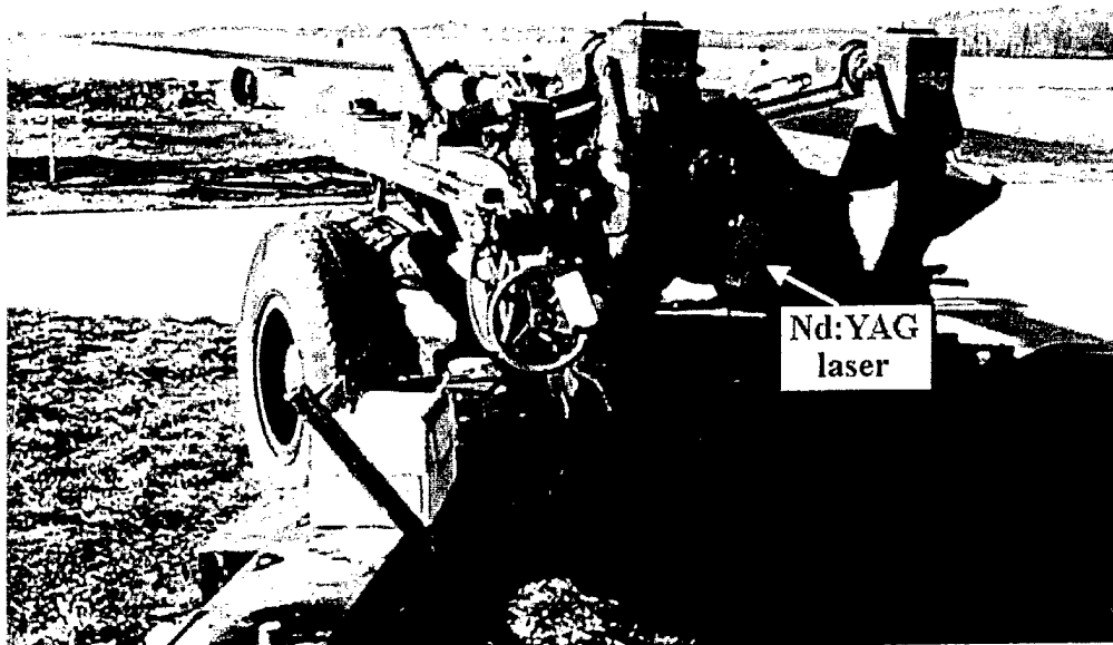
Figure 1. “Brick” Nd:YAG Pulsed Laser on M198 Cannon Breech During December 1997 Study.
