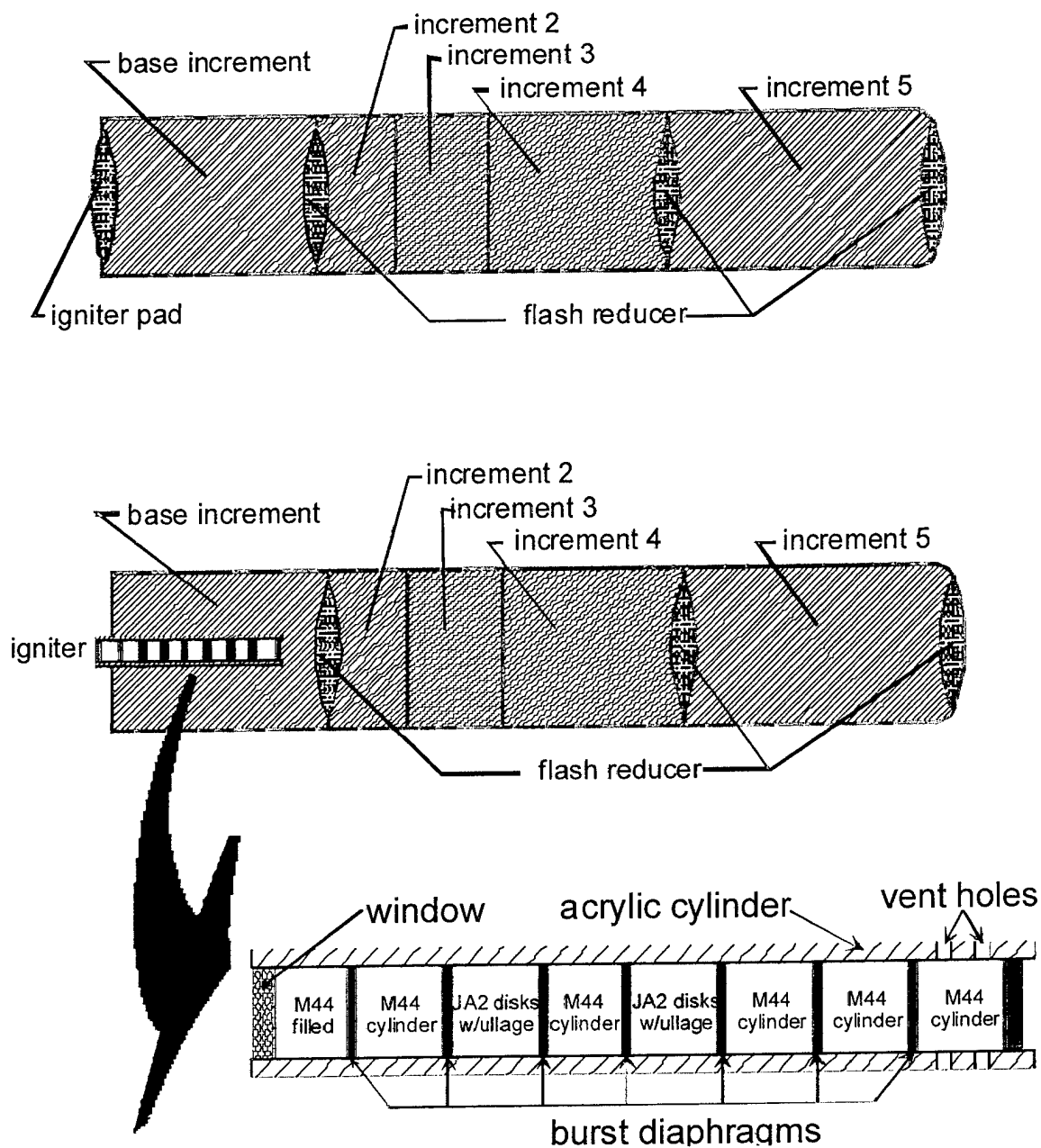
Figure 2. M3A1 Charge in Standard Configuration (upper) and With Modified Igniter (lower).
