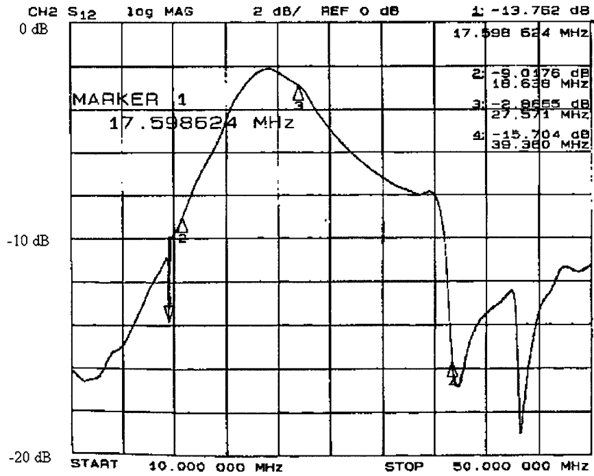
Fig. 5. Response of filter made in May 1998 shows lower insertion loss and high return loss, but with a widened bandwidth
