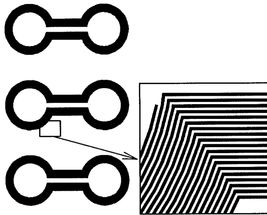
Fig. 6 A 3-spiral resonator
