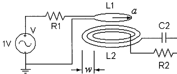
Fig. 13. Model of the self-resonant spiral resonator
