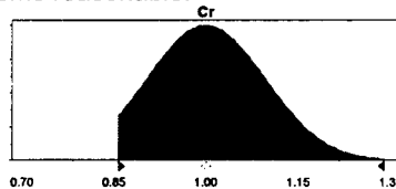
Figure 9. Distributions of Inputs Used in the Simulation
