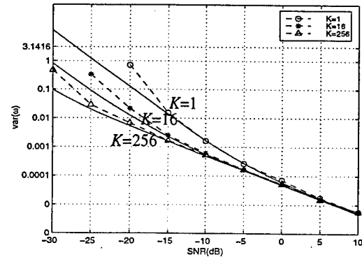
Fig. 3 Variance of estimation error vs SNR
