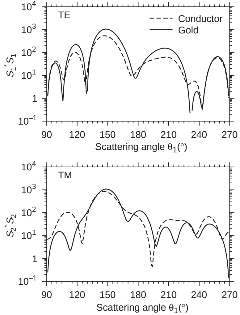
Figure 2. Light scattering intensities calculated for r = 0.55 \mu\text{m} spheres on a substrate illuminated at \lambda = 0.6328 \mu\text{m} , \theta_o = 30^\circ , \phi_1 = 0^\circ , and d = 0.55 \mu\text{m} . Results are shown when system is composed entirely of gold ( m_{\text{sph}} = 0.226 + 3.32i ) and when system is perfectly conducting.
