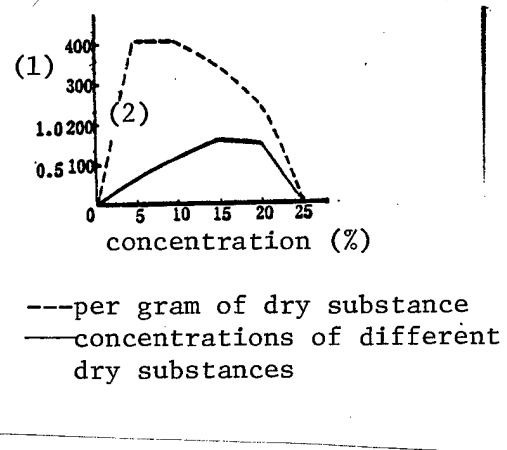
Figure 3. Relationship between the concentration of dry substance of commonly used raw material in rural areas and the amount of gas produced.
