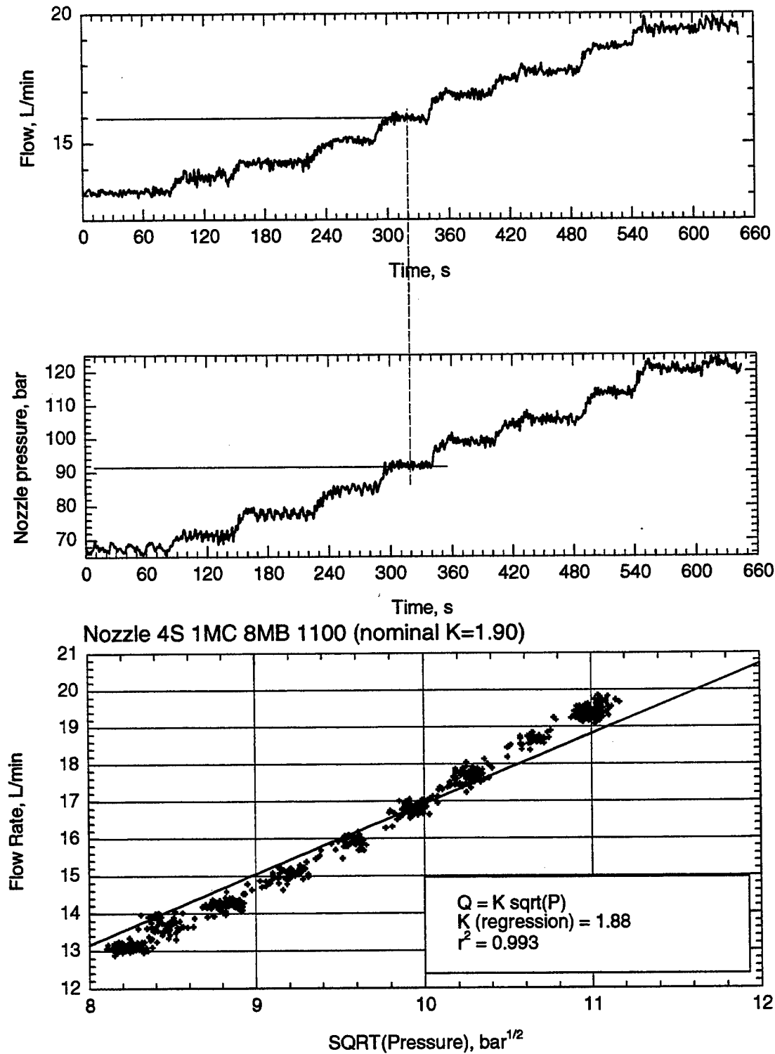
Marioff Nozzle, 4S 1MC 8MB 1100 at 103 bar
