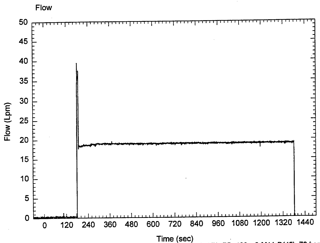
Plot 1. Pressure-Flow data for test T9MFC3
