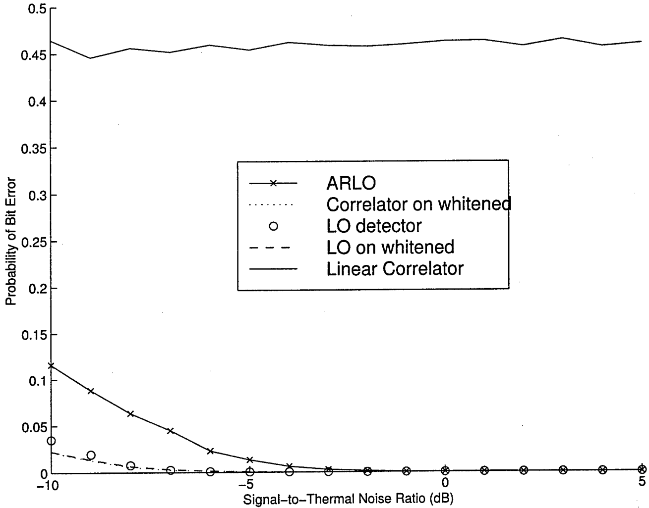
Figure 3: CW environment for the case of ISR = 30\text{dB} with PG = 12\text{dB}
