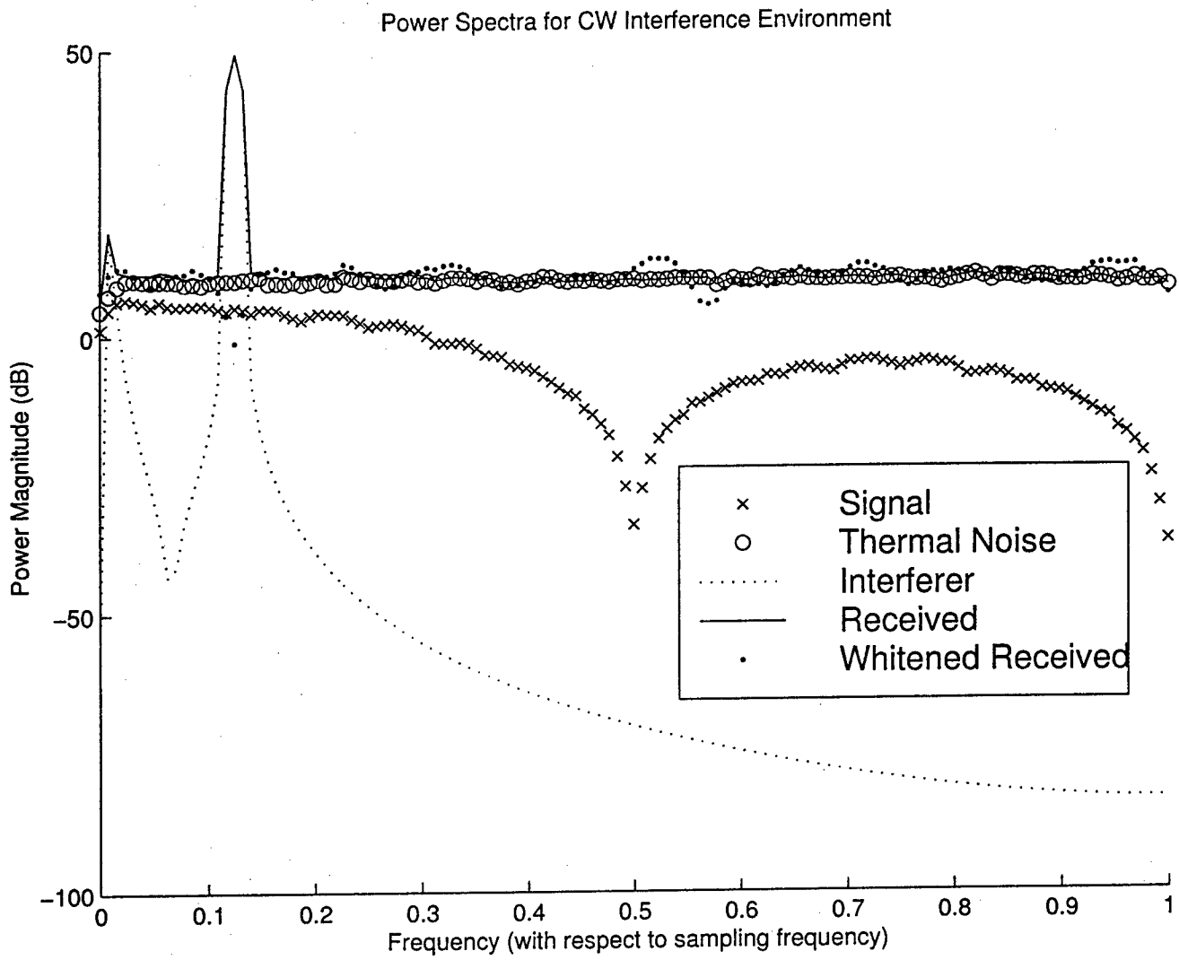
Figure 4: CW spectra for ISR = 30\text{dB} with PG = 12\text{dB}
