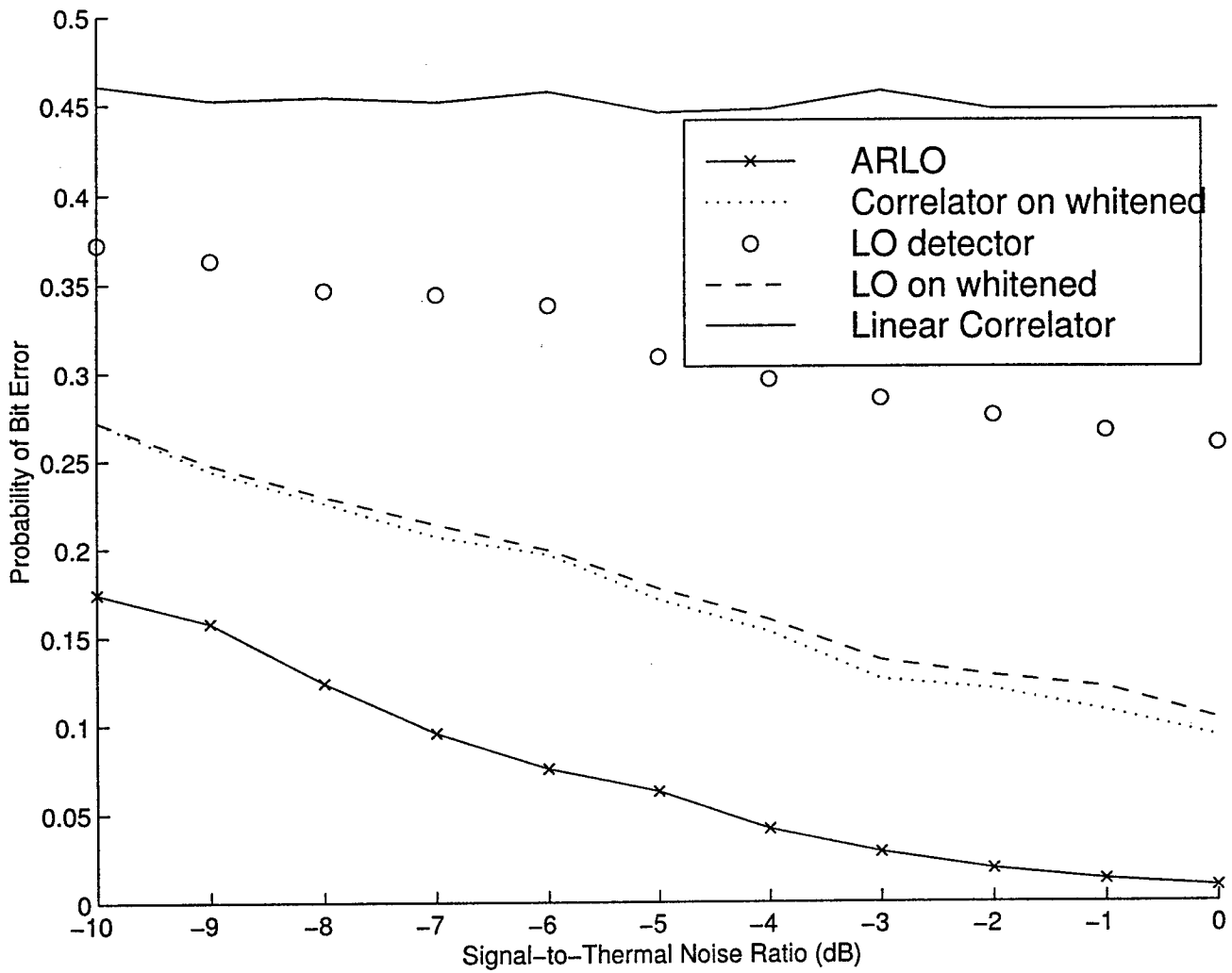
Detector Performance in Multi-CW Interference Environment
