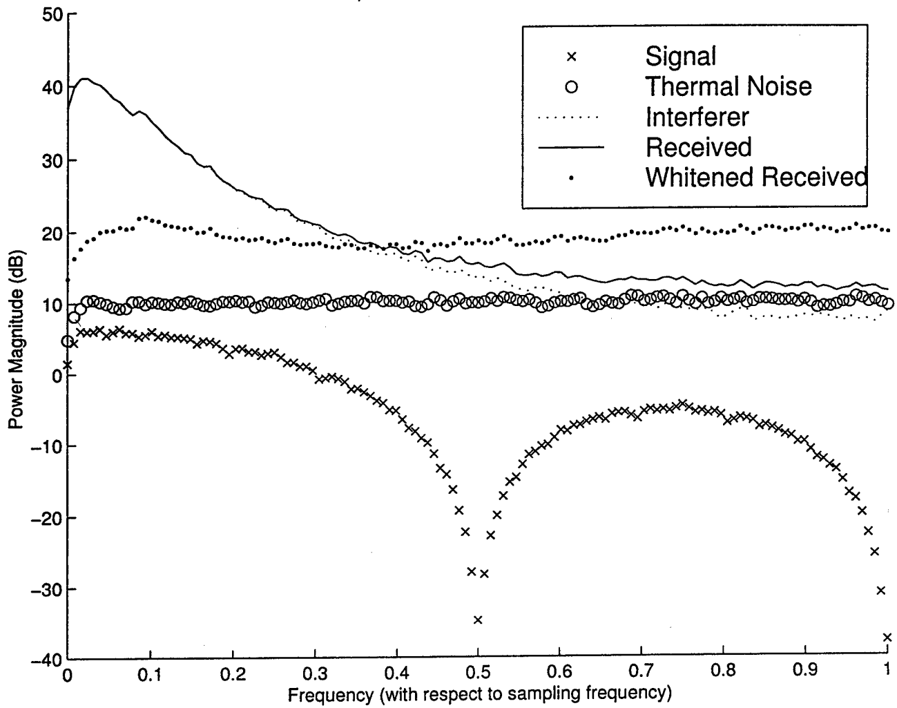
Power Spectra for PB Interference Environment
