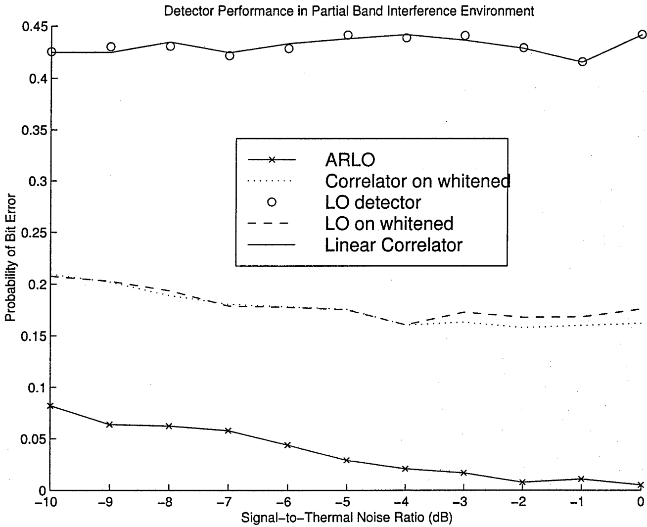
Figure 1: Partial Band environment for ISR = 30\text{dB} with PG = 12\text{dB}
