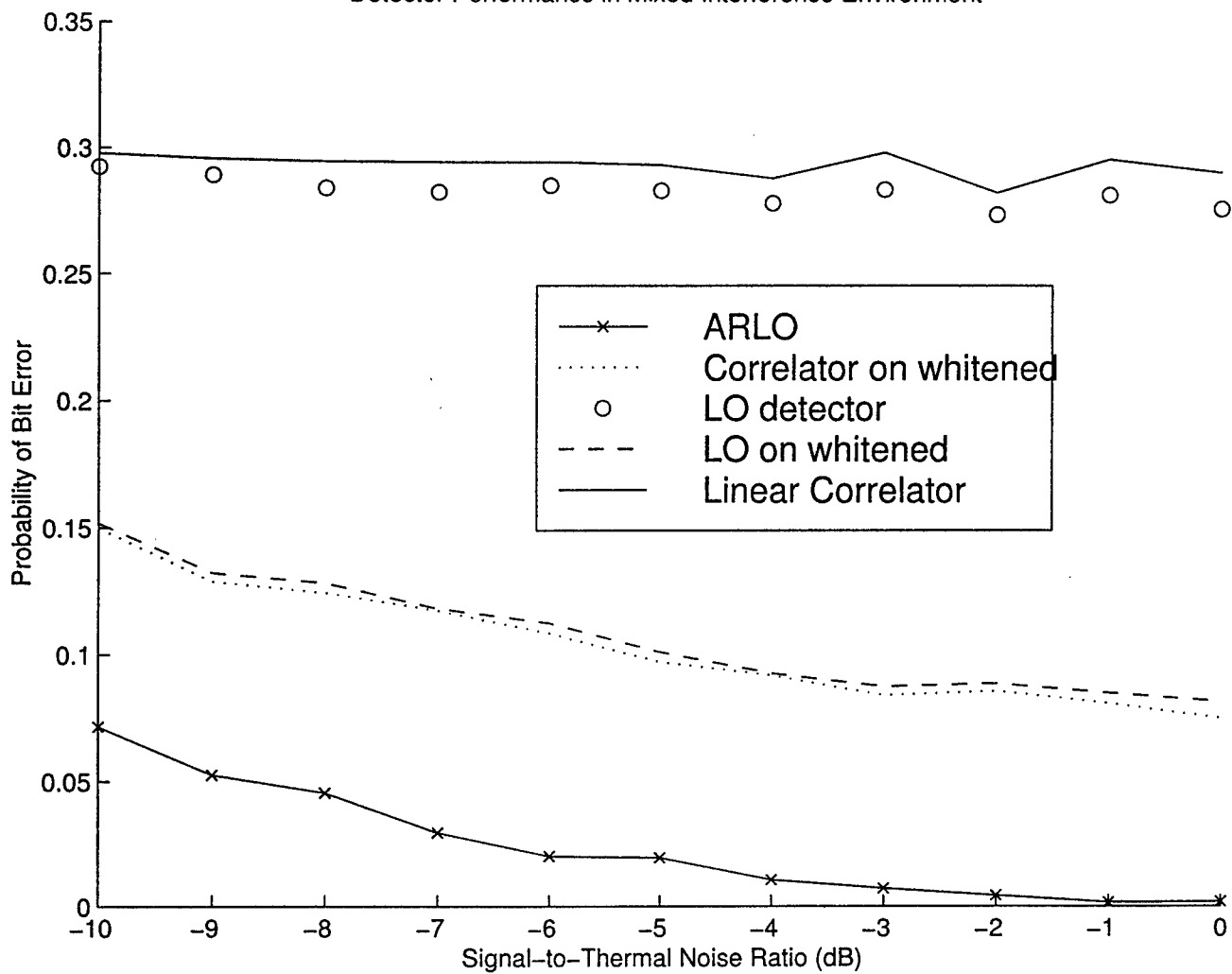
Detector Performance in Mixed Interference Environment
