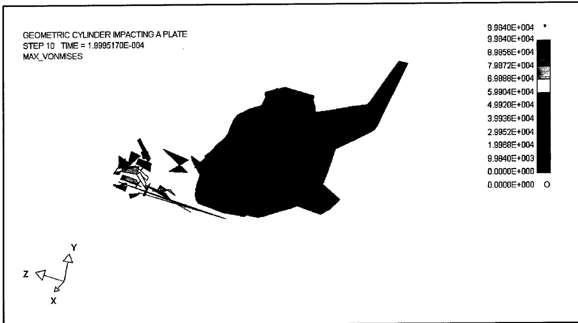
Figure 5. Helicopter Structure Hit by APFSDS Ammunition.
