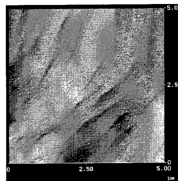
Fig. 1 AFM image of FIELO GaN surface grown at 120\ \mu\text{m/h} .
