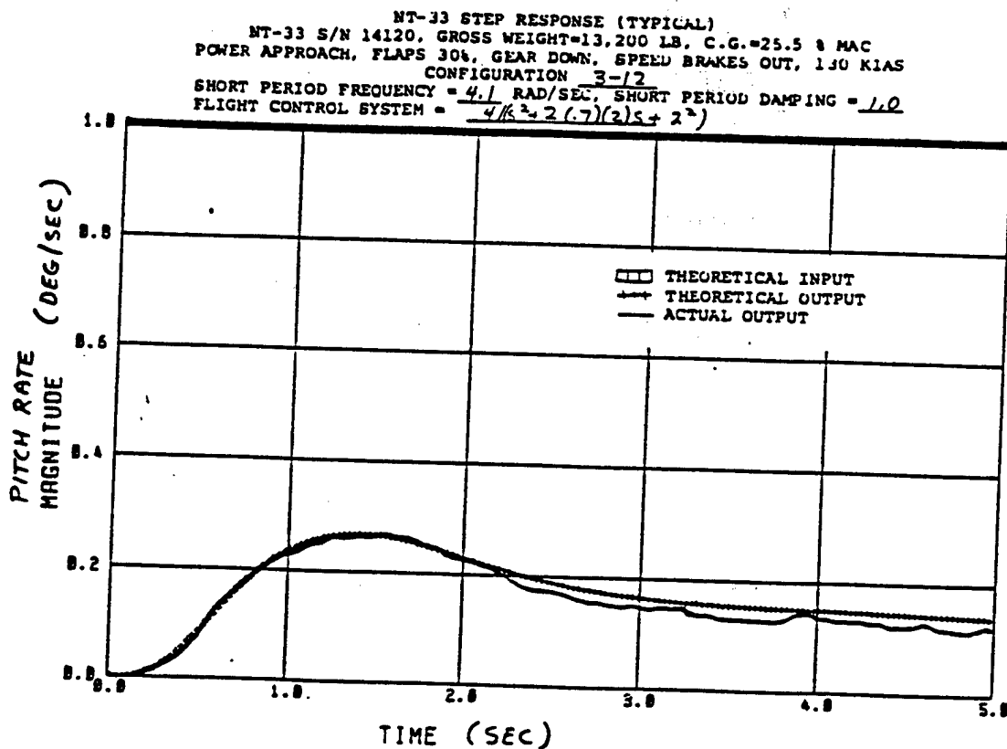
Figure D11. Step Response for Configuration 3-12.
