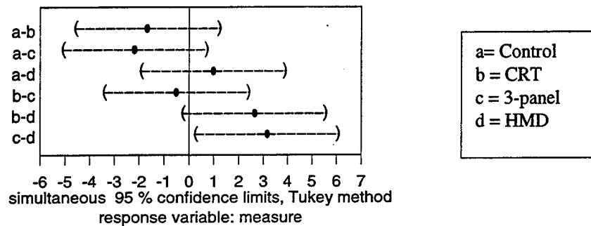
Figure 3- Tukey's method for honest significant differences for distance estimates
