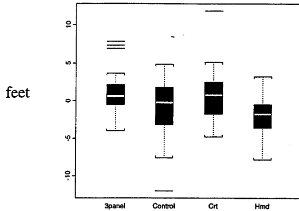
Figure 2- Box plot of distance estimation data
