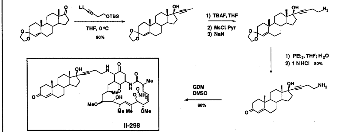
Figure 14. Synthesis of GM-dehydrotestosterone hybrid II-298.
