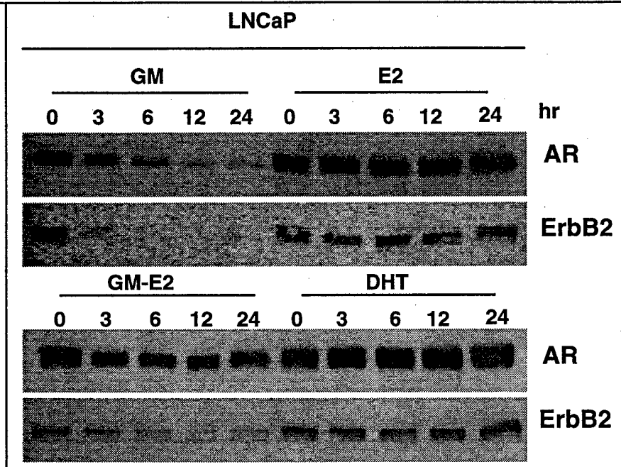
Figure 6. The GM-E2 hybrid compound II-211 inhibits the growth of human breast cancer cells. MCF7 and MDA MB-468 human breast cancer cells were treated with increasing drug concentrations. Cell number was determined after 5 days.
