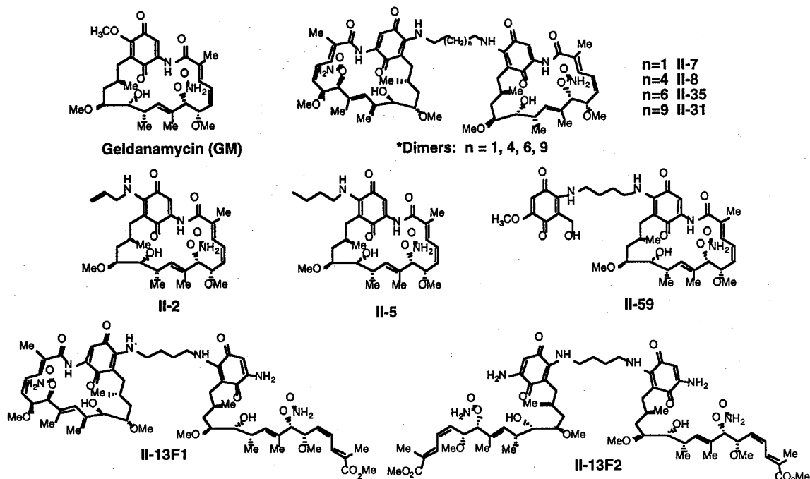
Figure 7. Chemical structure of geldanamycin dimers
