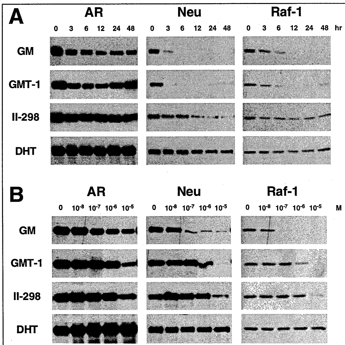
Figure 15. Effect of GM and GM-testosterone hybrids on the steady-state levels of cellular proteins on LNCaP human prostate cancer cells. A) LNCaP cells were grown in media supplemented with 1 \mu M GM, GM-DHT hybrids or dehydrotestosterone (DHT) for 0 to 48 hr. Cells were harvested and proteins were analyzed by immunoblotting using specific antibodies for androgen receptor, HER2/Neu or Raf-1. B) LNCaP cells were treated for 48 hr with various concentrations of GM, GM-DHT hybrids or DHT. Protein levels were analyzed as described for A).
