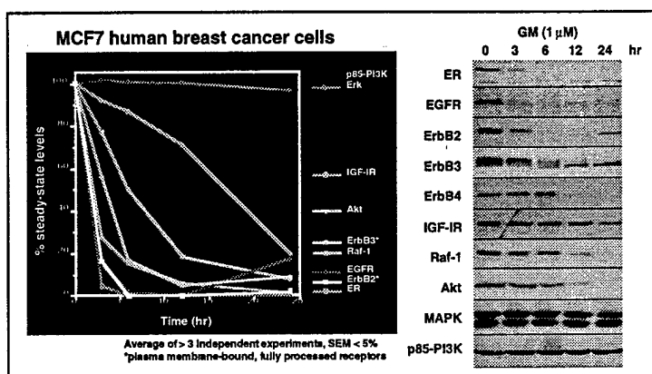
Figure 2. Changes in protein expression induced by GM. Most cellular proteins are not affected, heat shock proteins are upregulated. A specific set of proteins are decreased in response to GM. Decrease in steady-state levels in most cases, is mediated by enhanced degradation.
