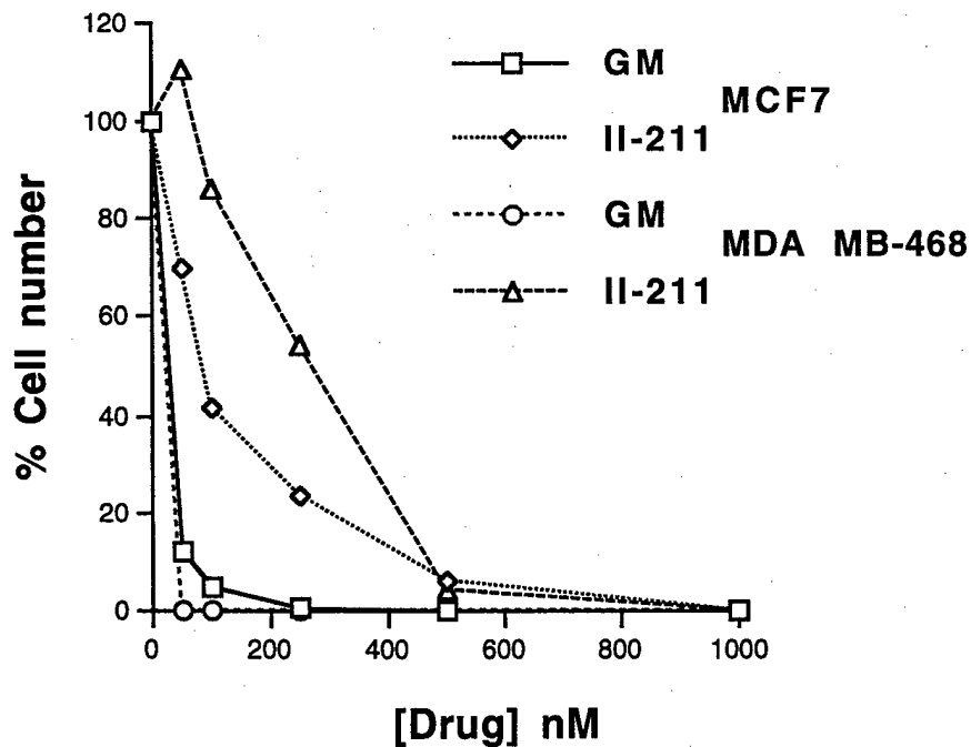
Figure 6. The GM-E2 hybrid compound II-211 inhibits the growth of human breast cancer cells. MCF7 and MDA MB-468 human breast cancer cells were treated with increasing drug concentrations. Cell number was determined after 5 days.
