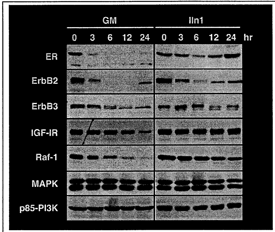
Figure 8. Effect of GM and GM-4C (II7, IIn1) dimer on the steady-state of MCF7 cellular proteins. MCF7 cells were treated for increasing time periods with 1 \mu M drug. Cells were harvested and SDS-protein extracts were analyzed by SDS-PAGE. The steady-state levels of several GM-targets were analyzed by immunoblotting with specific antibodies.
