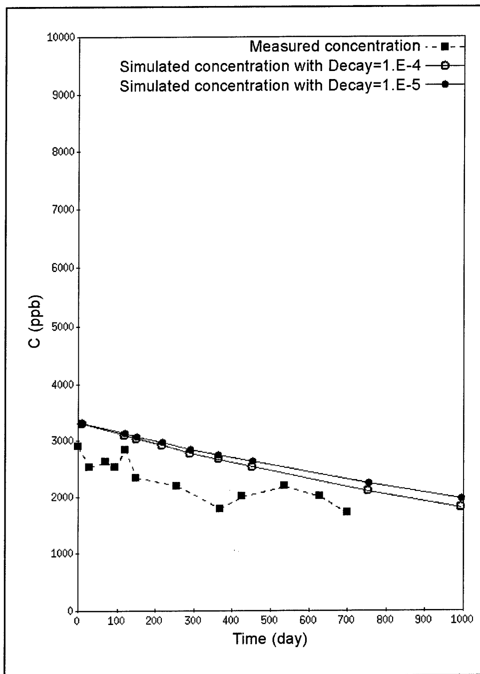
Figure 14. Time series of TNT concentration for measured and calibrated model with different first-order decay rates ( 1.E-4 and 1.E-5 1/day) and fixed adsorption coefficient of 2.3E-1 L kg -1 as shown above (Original data were from MW083U)
