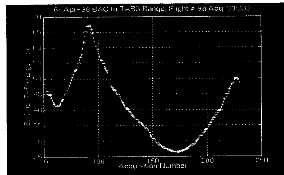
(f) TARS-to-BAC 1-11 Range
