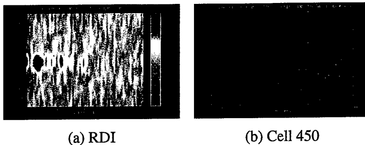
Figure 2-21. JDL_1x6 = (0*0)x(3*2) Algorithm Applied to Acquisition #5-152, Angle Index 58; Channels: 22; Support Cells: (-20, +10); Guard Cells: ±3
