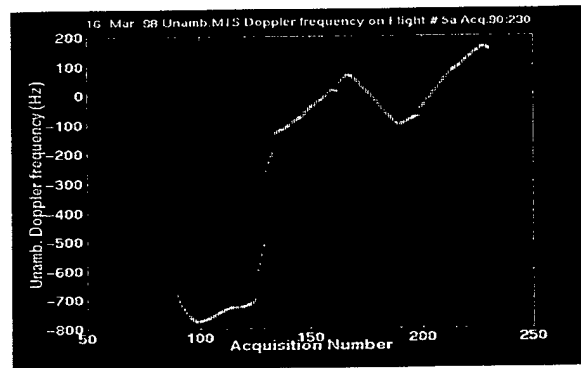
(l) Doppler Shift of MTS Tones
