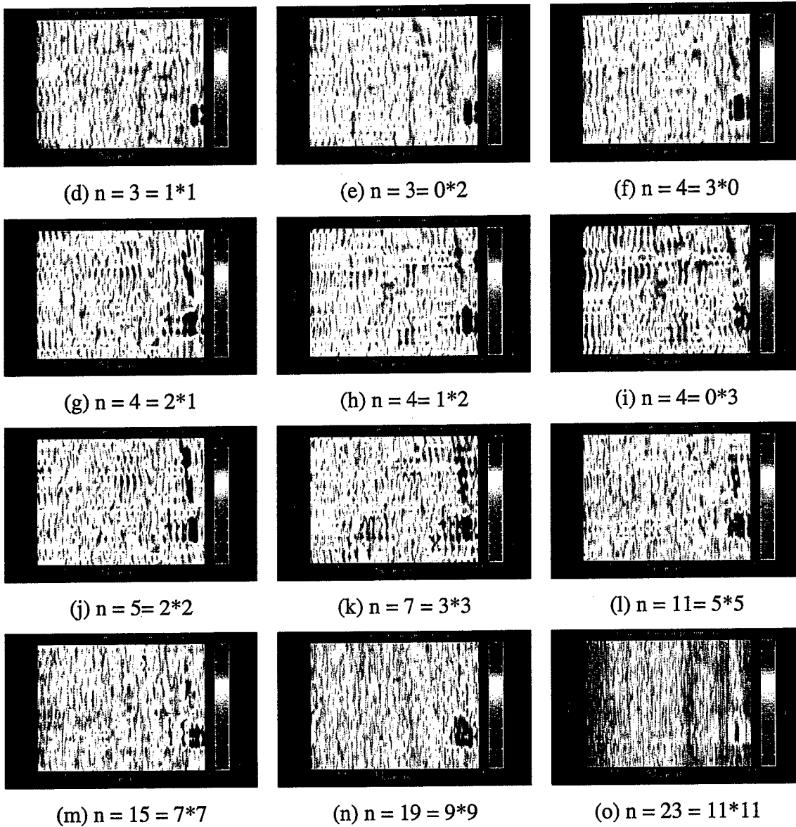
Figure 3-14. JDL 1 \times n -Adapted RDI, Acquisition #9-110 (Channels: 22; Support Cells: -20,+10; Guard Cells: \pm 3 ) (Concluded)
