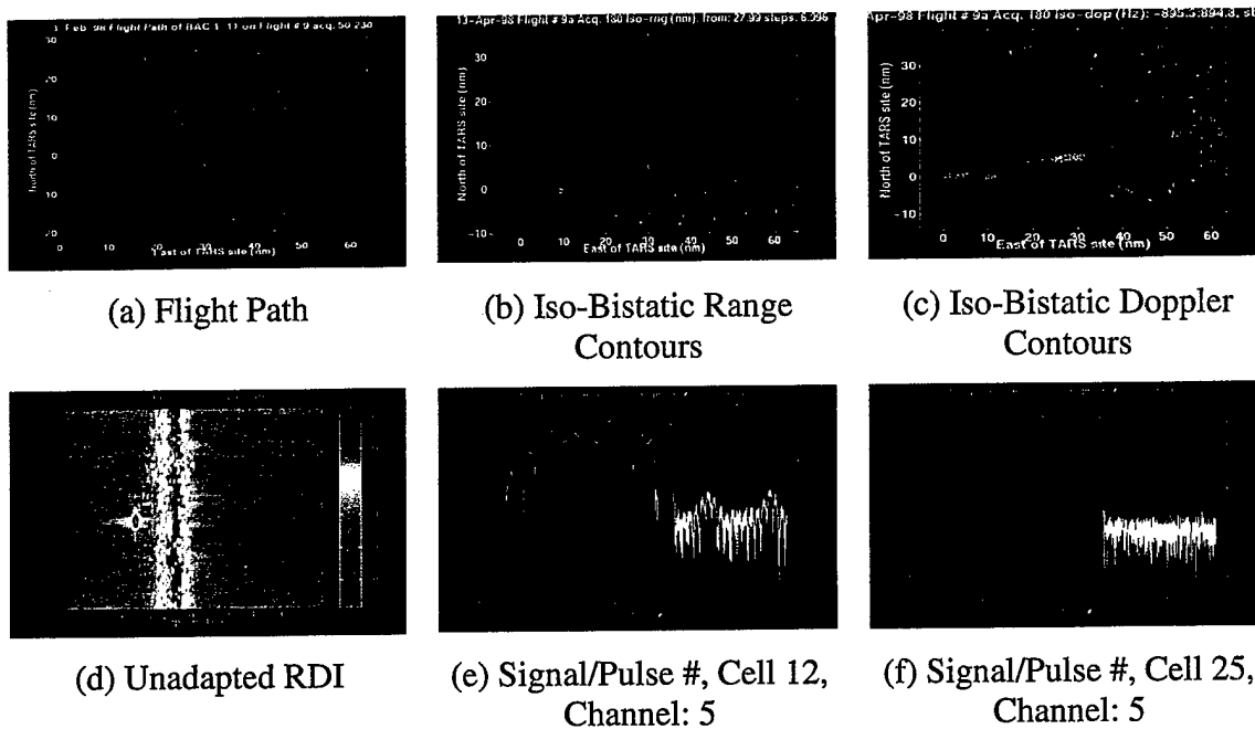
Figure 3-20. Pseudomonostatic Acquisition #9-180
