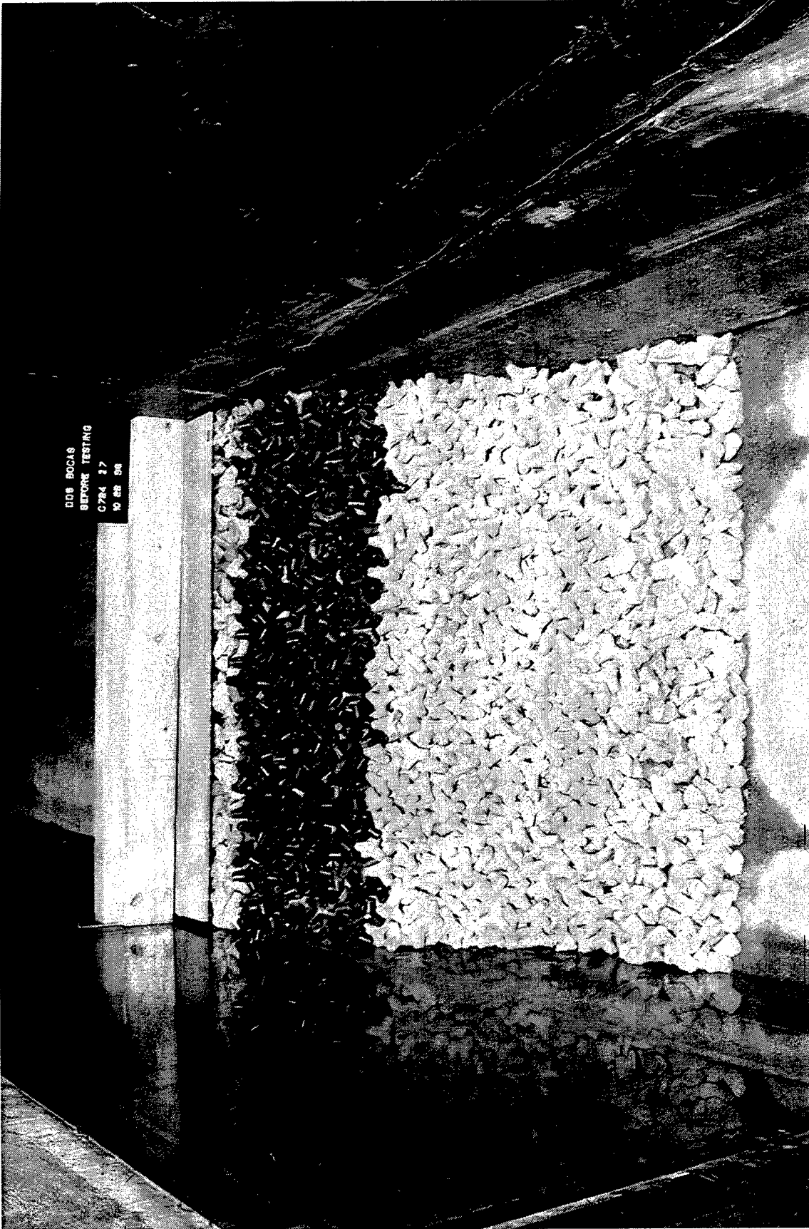
Photo 27. Harbor-side view of Plan 2 before wave attack
