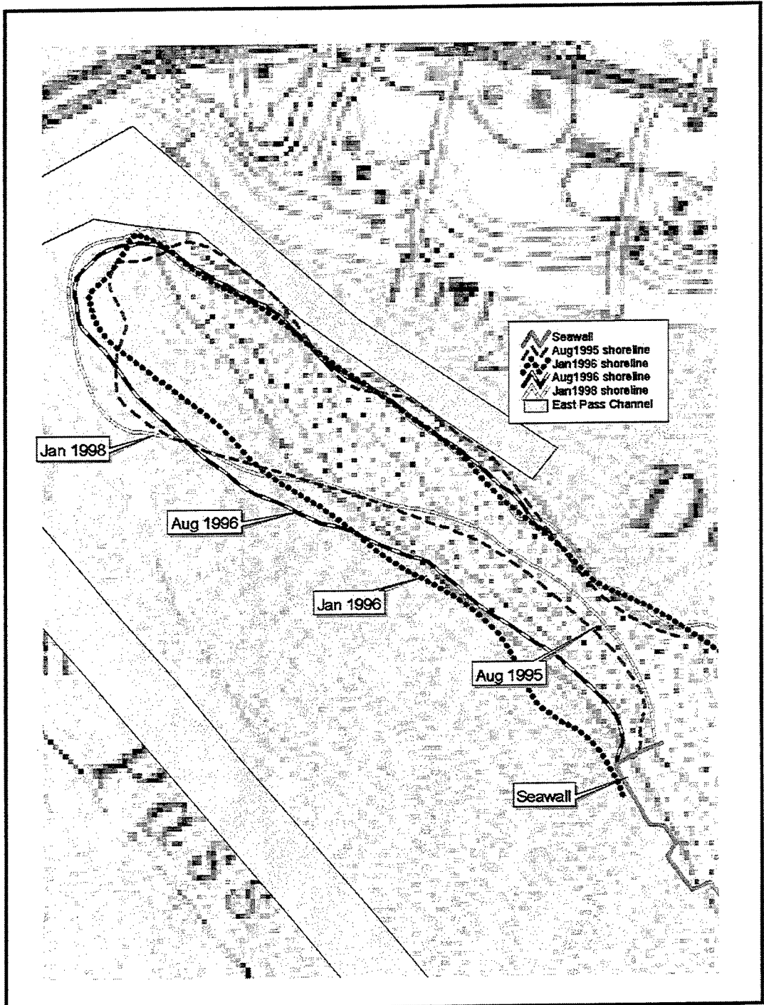
Figure 8. Norriego Point shoreline evolution
