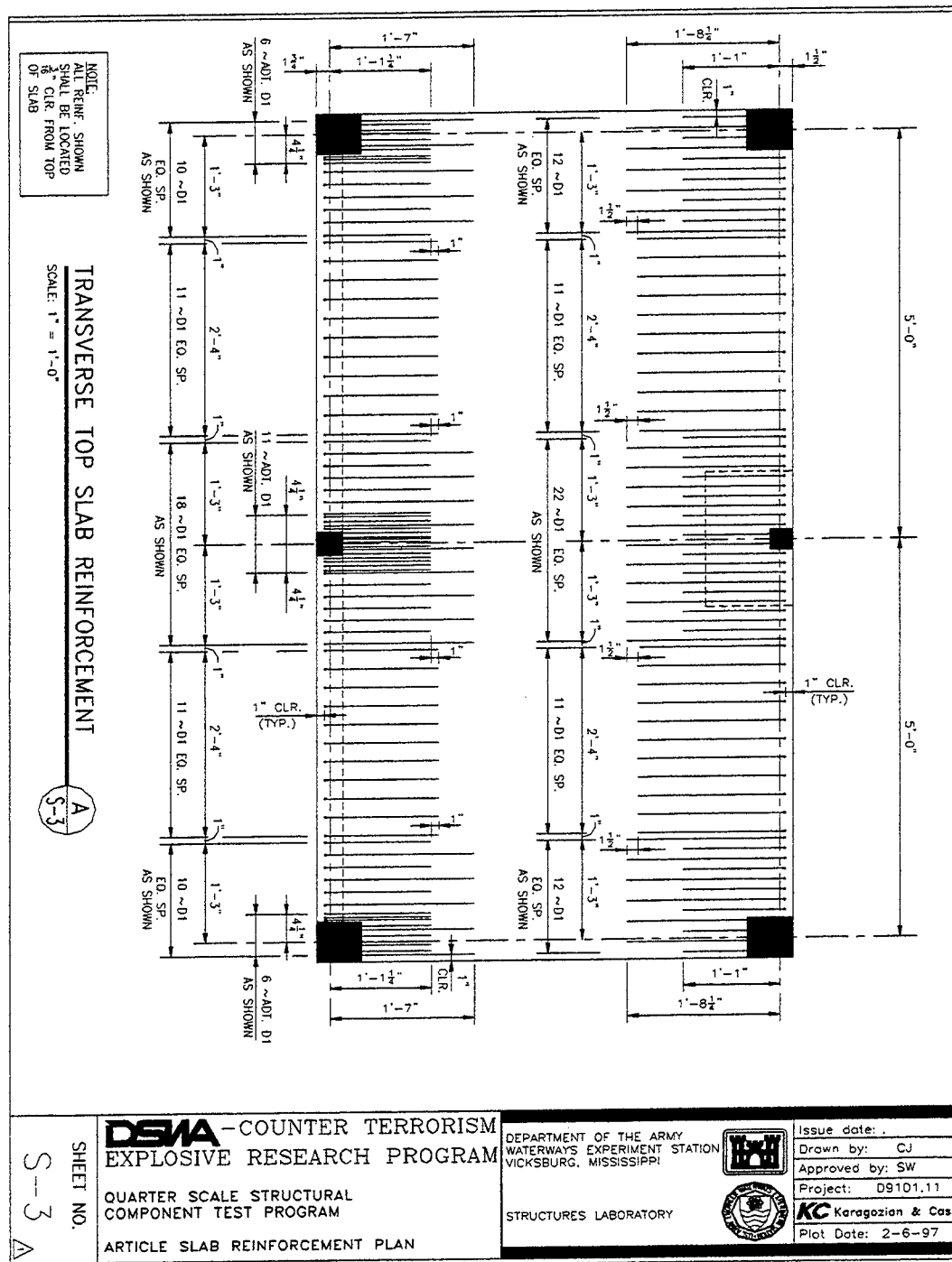
Figure 2.5 Slab Reinforcement Details, Top Transverse
