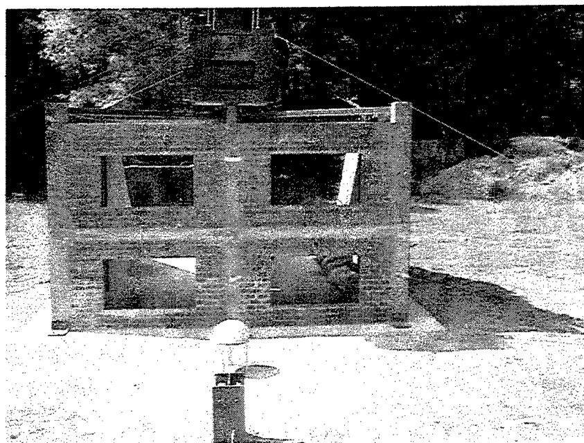
Figure 2.20 Pretest View, Experiment No. 4
