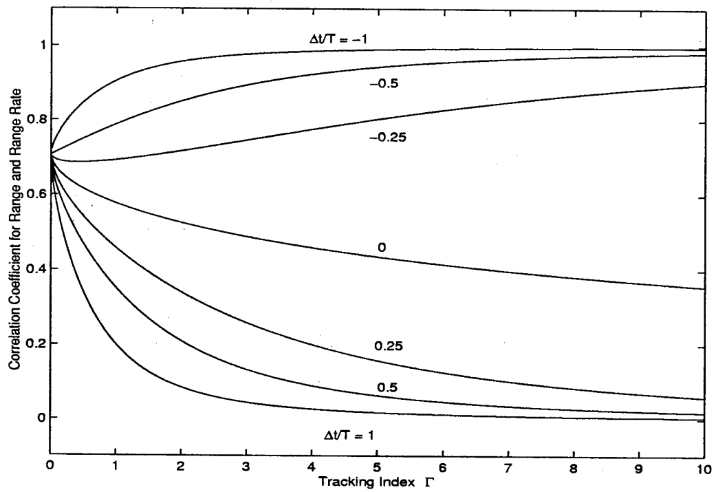
Figure 2. Correlation Coefficient for Range and Range Rate Versus \Gamma with T = 1 s and \sigma_v = 10 m
