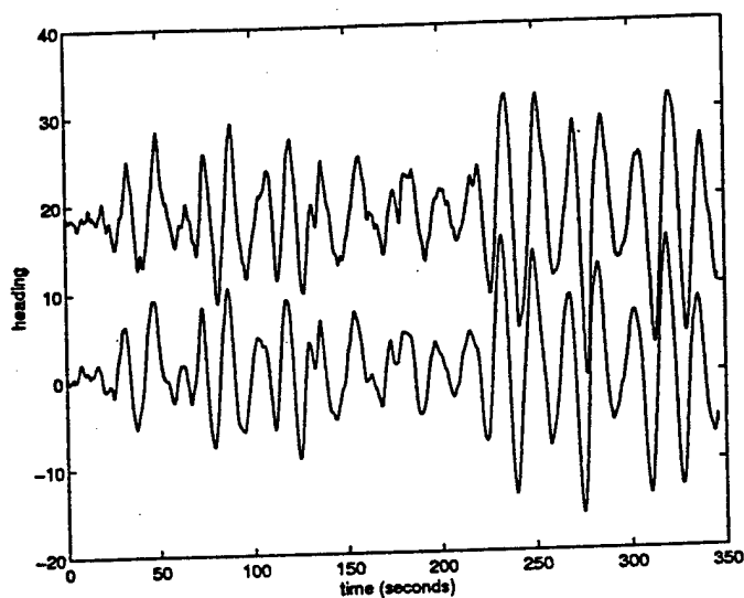
Figure 1: Raw heading from POS/MV and fluxgate compass.
