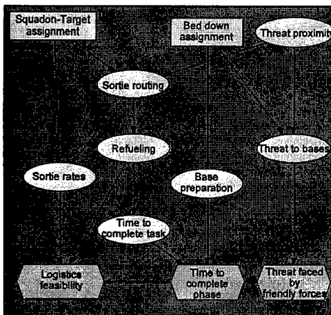
Figure 2. Influence Diagram.
