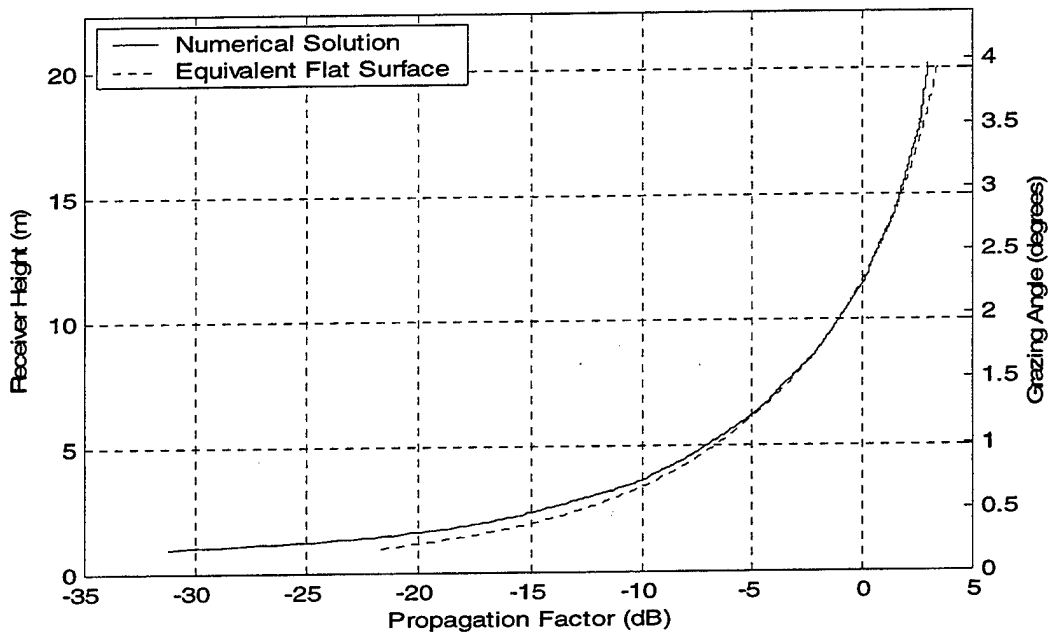
Figure 39: Upper Figure: Equivalent Impedance of Sinusoidal Surface with Period = 30 m and Peak to Peak Amplitude = 1 m. Total Distance = 300 m. Frequency = 1 GHz. Antenna Height = 1.5 m. \Delta x = 0.3\text{m} . One hundred realizations. Lower Figure: PF for the PEC Sinusoidal Surface Above and for the Equivalent Flat Lossy Surface.
