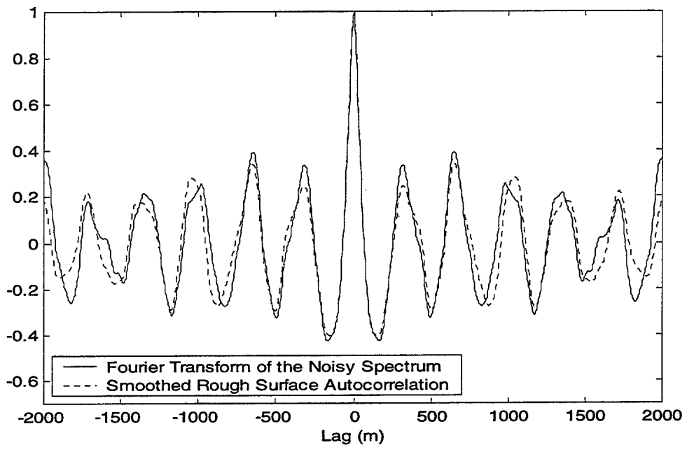
Figure 45: Normalized Fourier Transform of the Noisy Spectrum and Rough Surface Autocorrelation (Upper Figure) and Normalized Fourier Transform of the Noisy Spectrum and Smoothed Rough Surface Autocorrelation (Lower Figure). Wind Speed = 20m/s
