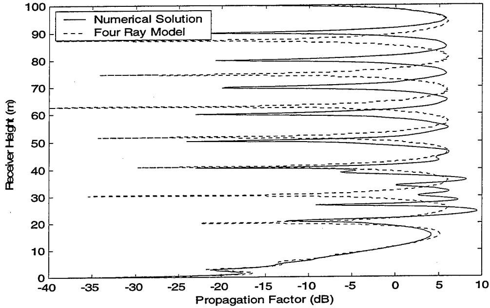
Figure 15: Total Current and Incident Current (Upper Figure) and Propagation Factor (Lower figure) for the Triangular Hill with a = b = c = d = 50 m, Peak Height = 5 m and Antenna Height = 3 m. Frequency = 1 GHz. Calculation in one section. \Delta_x = \lambda .
