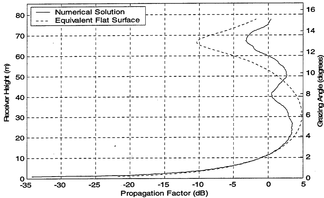
Figure 40: Upper Figure: Equivalent Impedance of Sinusoidal Surface with Period = 30 m and Peak to Peak Amplitude = 1 m. Total Distance = 300 m. Frequency = 1 GHz. Antenna Height = 1.5 m. \Delta x = 0.3m . Fifty realizations. Lower Figure: PF for the PEC Sinusoidal Surface Above and for the Equivalent Flat Lossy Surface.
