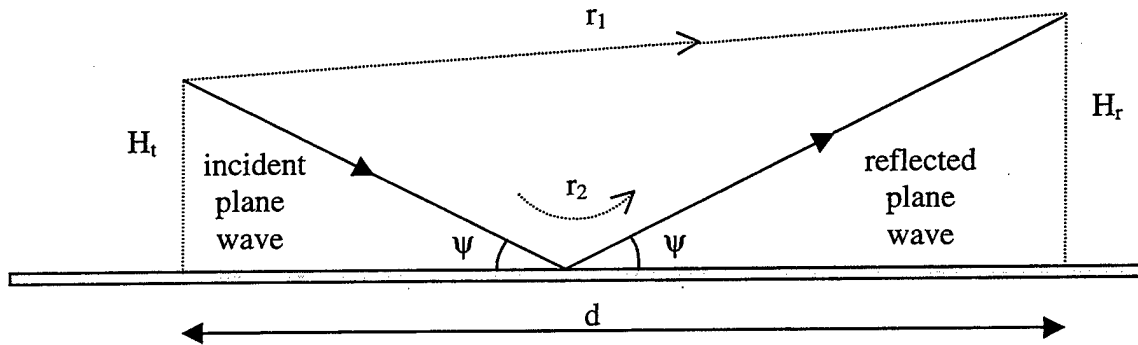
Figure 5: Reflection of Plane wave over Flat Surface
