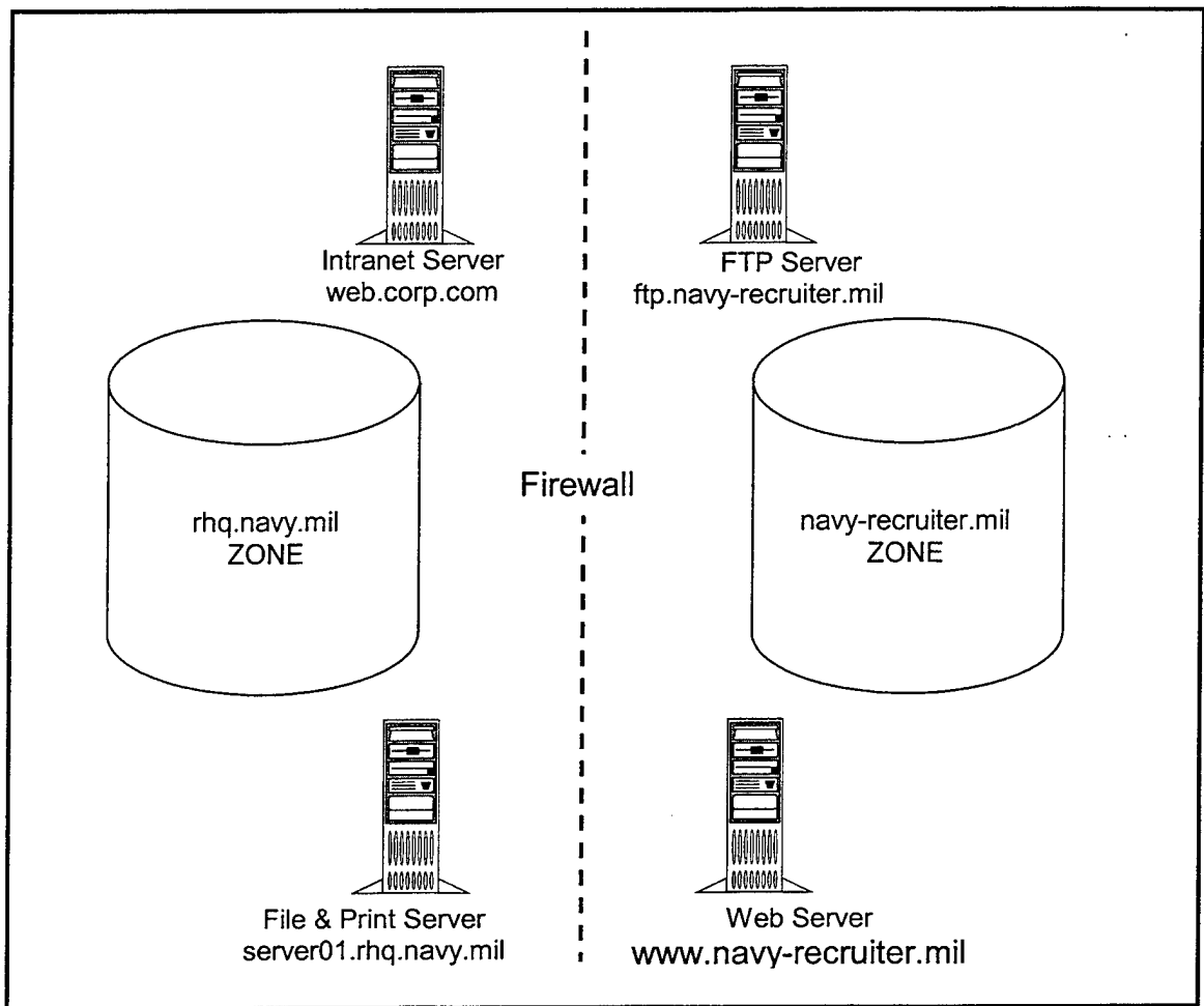
Figure 4.4. Different internal and external namespaces used in a network. After Ref. [21]
