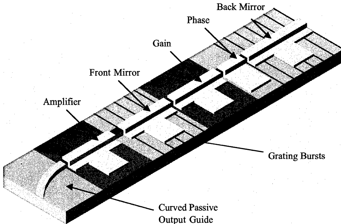
Figure 5. SGDBR laser with integrated semiconductor optical amplifier.
