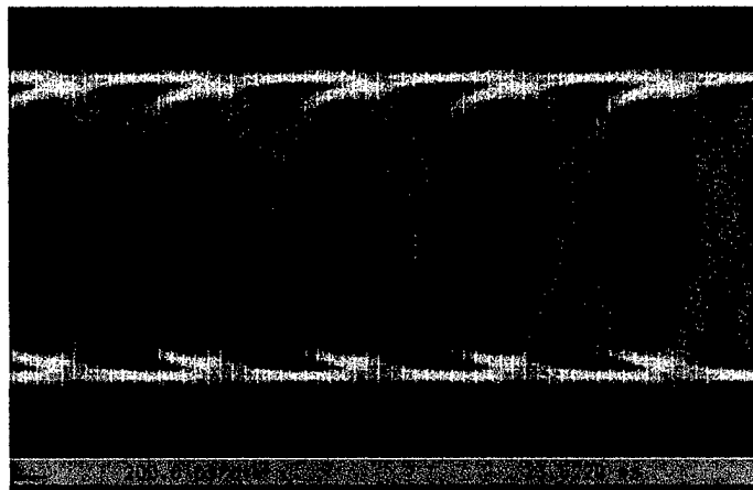
Figure 10. Eye Diagram at 2.488 Gbit/s Data Rate, 2^{31}-1 Pattern Length and 1E-9 Error Ratio
