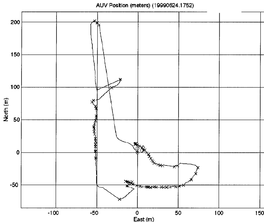
Figure 3.2.3.2 : Docking Run
