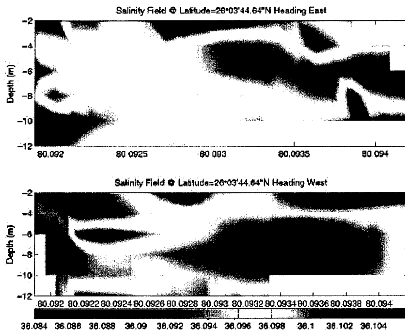
Figure 3.2.1.10. Salinity field at constant latitudes for longitudinal legs. Note variation of salinity O(0.1 \text{ psu}) .
