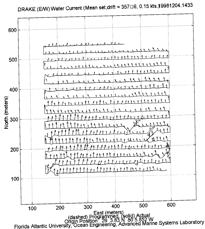
Figure 3.1.4: Current measured on mission 19981204.1433.
