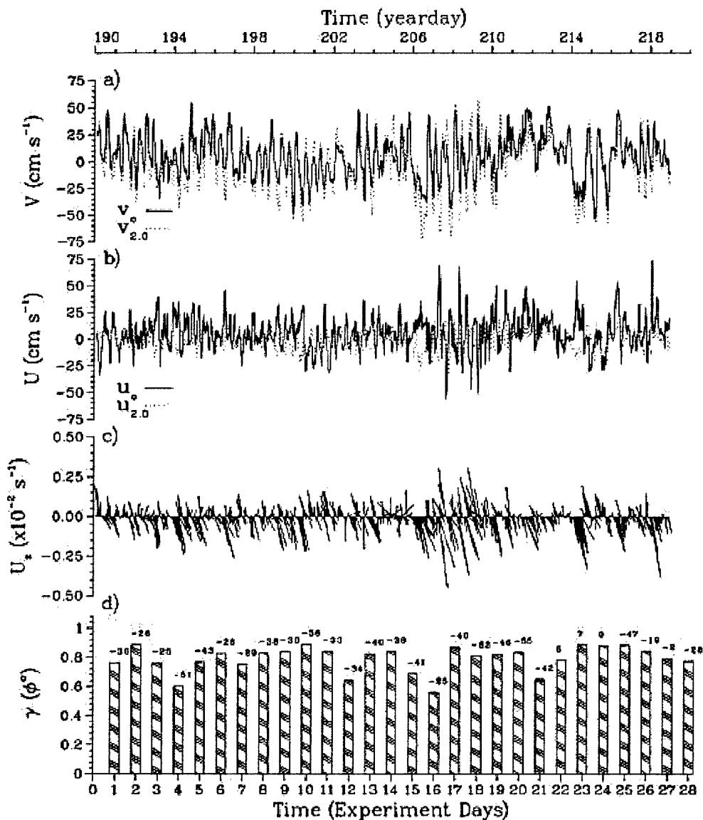
Figure 3.3.5: Comparison of OSCR-derived surface and subsurface current time series at the 10 m mooring deployed by NOVA and USF for the a) v-component ( \text{cm s}^{-1} ), b) u-component ( \text{cm s}^{-1} ), c) current vector shear ( \times 10^{-2} \text{ s}^{-1} ), and d) daily complex correlation coefficients (and phases) relative to the surface velocity. A negative phase implies a clockwise veering of the current with depth. The subsurface data was provided by Alexander Soloviev (NOVA) and Robert Weisberg and Mark Luther (USF).
