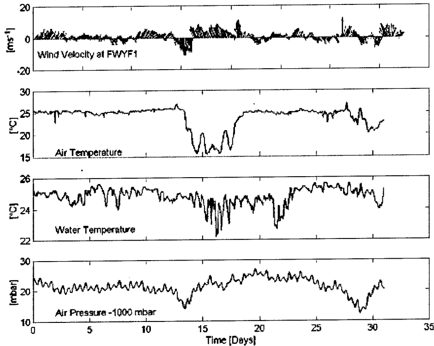
Figure 3.2.1.4. Atmospheric conditions recorded by NOAA C-MAN buoy at Fowey Rocks during December.
