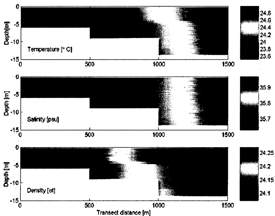
Figure 3.2.1.5b. Composite views of temperature, salinity and density during Dec. 17 over a transect along 26^{\circ} 3.8' N starting at 26^{\circ} 3.8'N 80^{\circ} 5.68'W .
