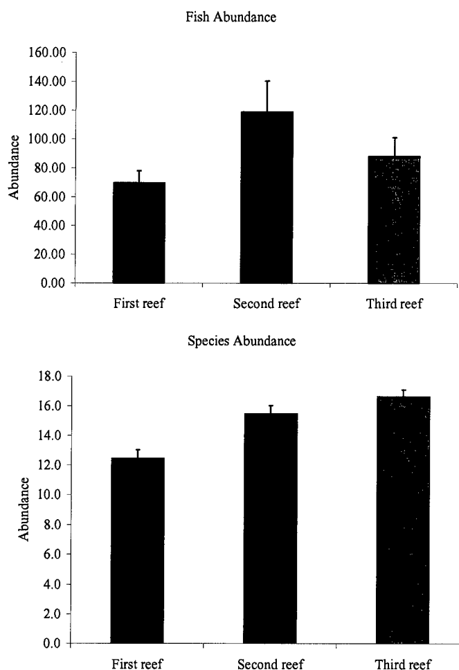
Figure 3.6.3.2: Fish abundance and species (mean \pm 1SE) for each of the three reefs within the range. Letters above columns indicates significant difference between the means ( p < 0.05 , SNK).
