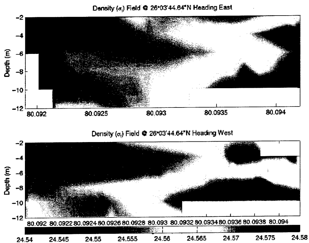
Figure 3.2.1.12. Density field consistent in each direction.
