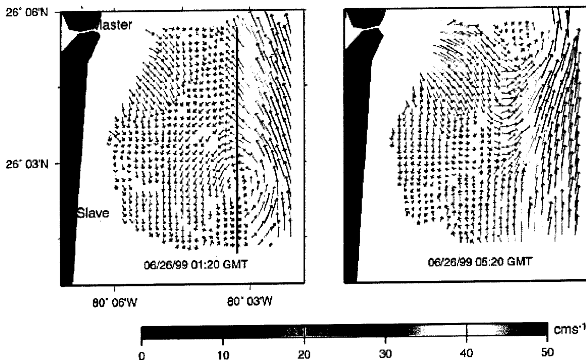
Figure 3.3.2. Surface current images from the SFOMC 4-D Current Experiment on 26 June: at 0120 GMT (left panel) and 0520 GMT (right panel). The black solid line represents a transect described below.
