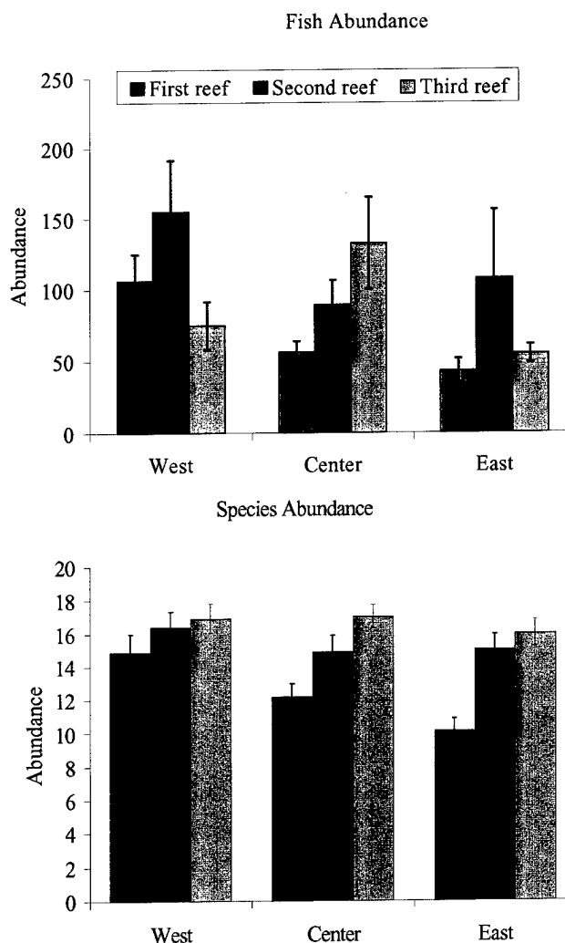
Figure 3.6.3.3: Fish abundance and species (mean \pm 1SE) for each of the three sample locations for each of reefs within the range.
