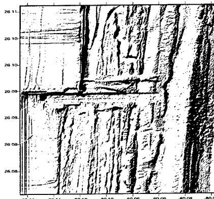
Figure 3.6.3.5: Shaded surface plot of Port Everglades LIDAR.
