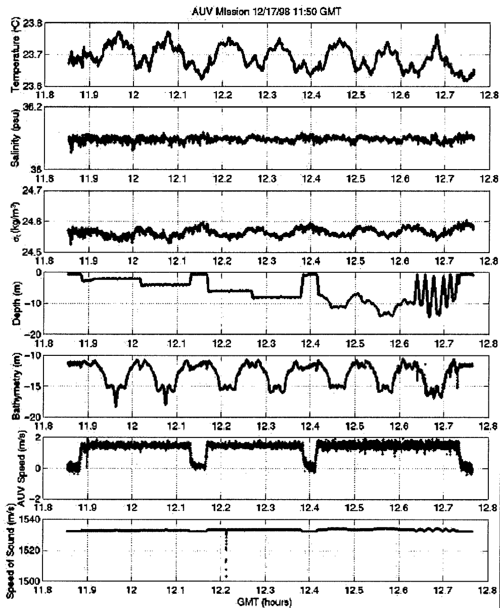
Figure 3.2.1.15. Time series data recorded by the OEX on Dec. 17.
