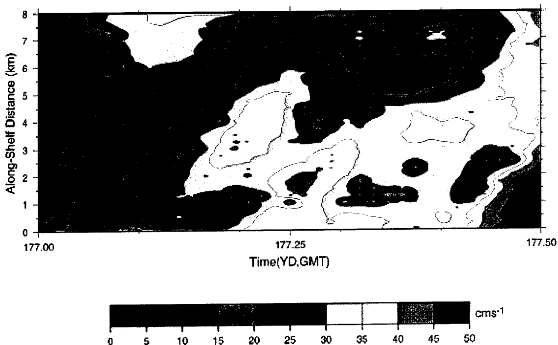
Figure 3.3.6: Along-shelf time section of surface current speed for a 12 h period on 26 June following the ring through the VHF domain. The path of the ring, as depicted by the near-zero current speed, has an approximate slope of 30 \text{ cm s}^{-1} with the current speed scale (color bar) as in Fig. 2.
