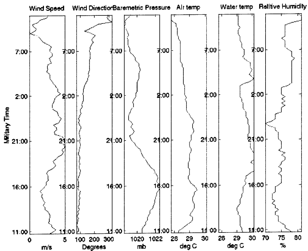
Figure 3.2.2.6: Weather data corresponding to the 24hr mission started on 07/21/99
