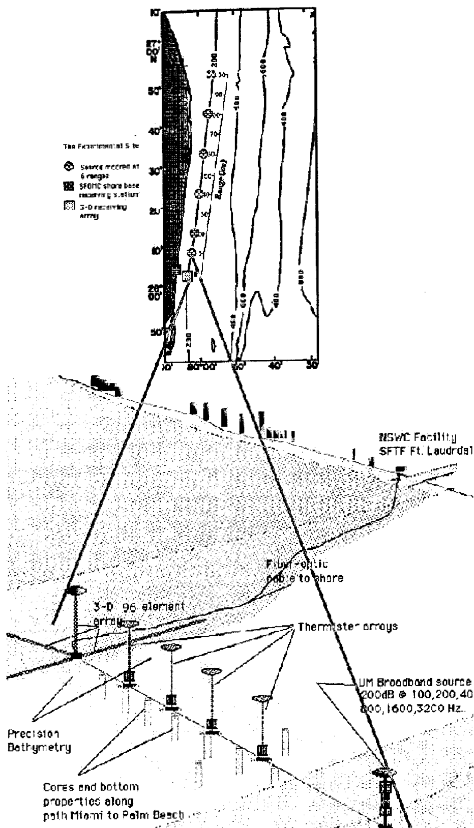
Figure 3.5.1. The SFOMC Acoustic Propagation Range
