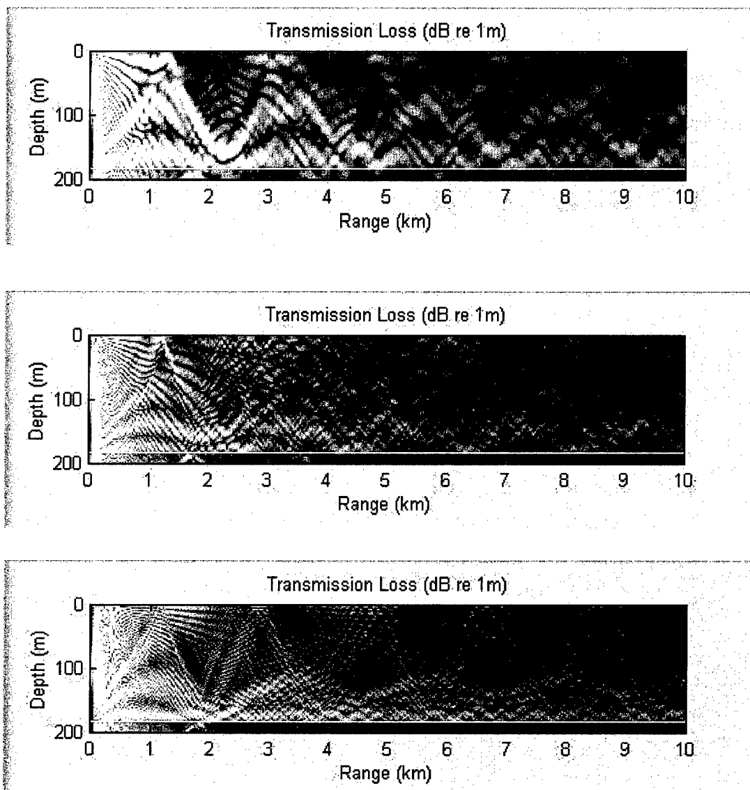
Figure 3.5.4 a-c Sound Field For Center Frequencies – Winter Profile.
