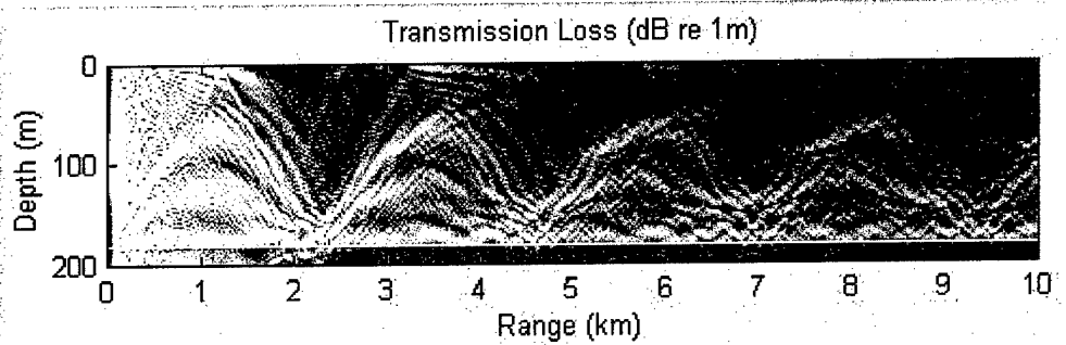
Figure 3.5.3 a-c Sound Field For Center Frequencies – Summer Profile.
