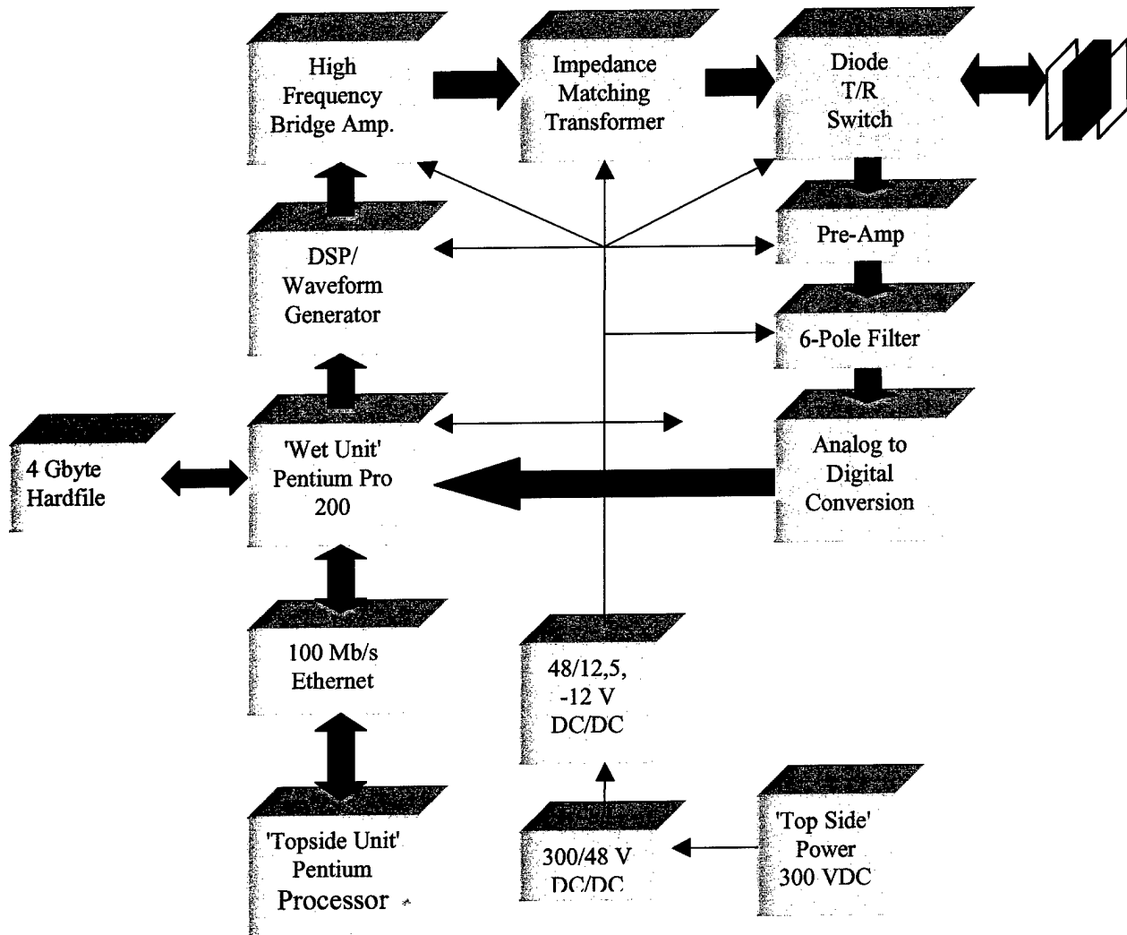
Figure 3.1.9: Block Diagram of 1.2 Mhz Chirp Sidescan Sonar
