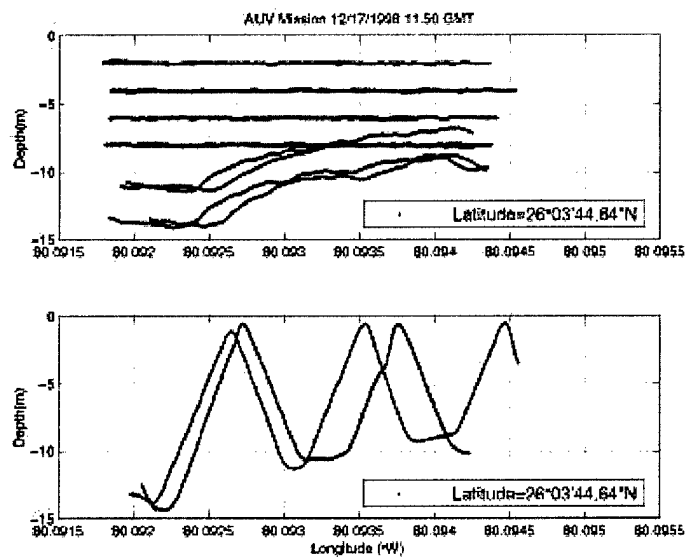
Figure 3.2.1.9. Mission path for the OEX.
