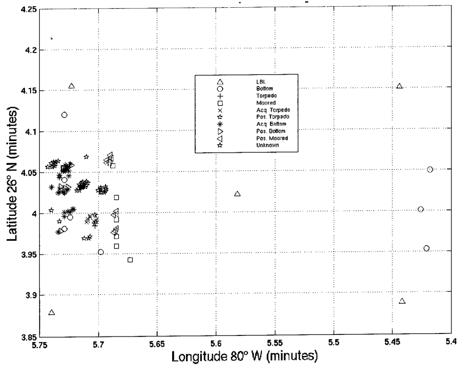
Figure 3.1.7: Mission 19981211.1630. Target plot showing detections and actual locations of targets.
