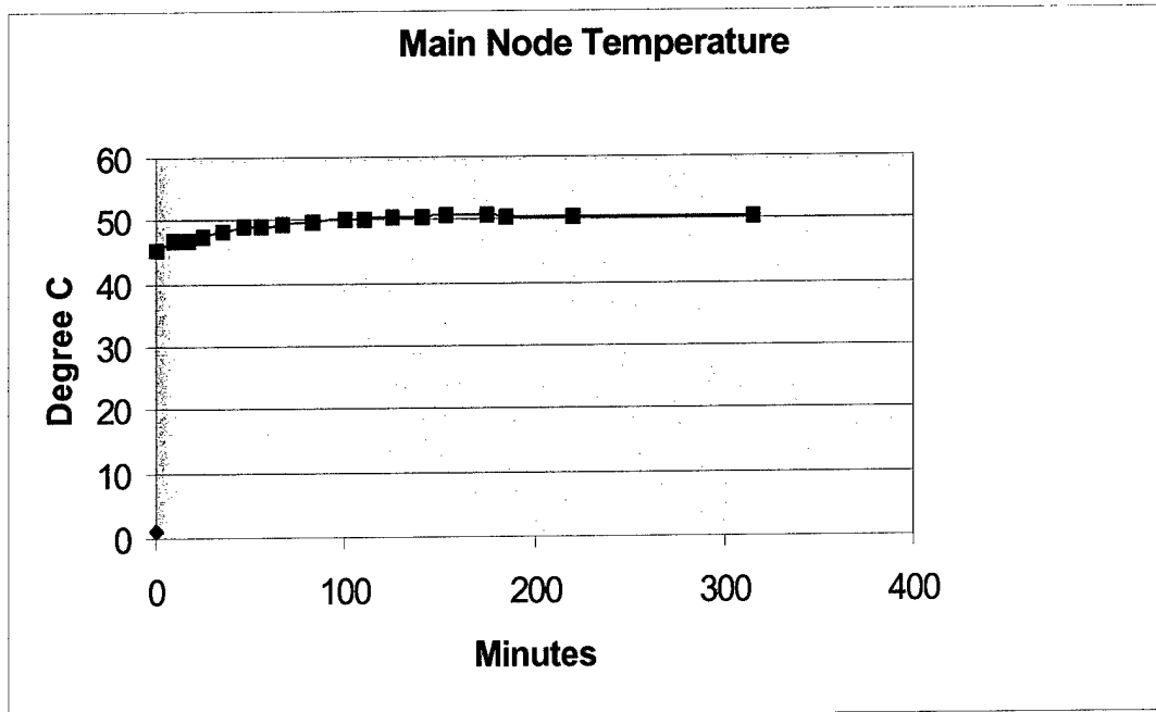
Figure 2.7.13 Internal MUX temperature fluctuation when subjected to close to 100% of maximum power load
