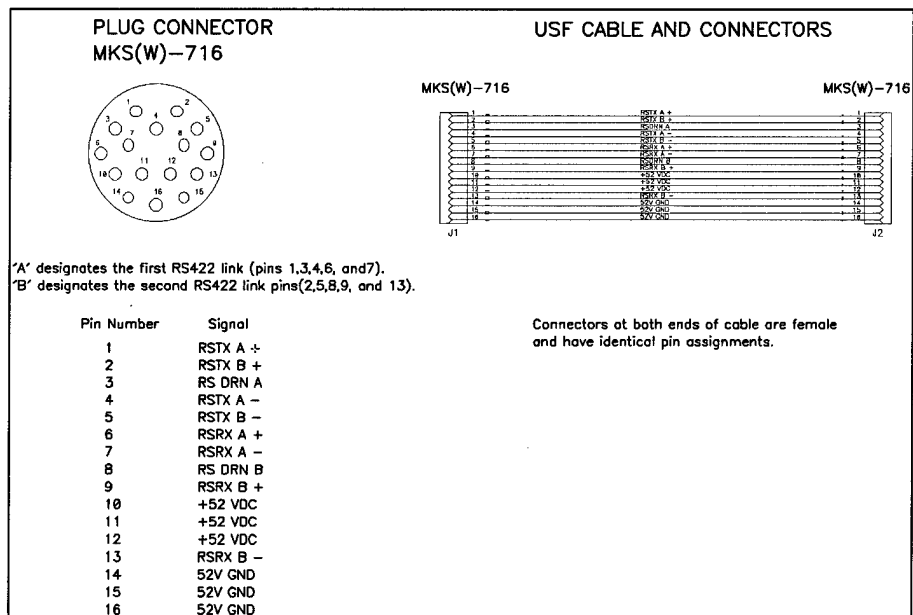
Figure 2.7.5 USF environmental array cable/connector pinouts
