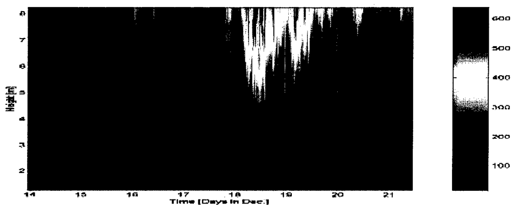
Figure 3.2.1.6: TKE ((\text{cm/s})^2) distribution in the water column over the 5-head ADCP during Dec 14 – 22, 1998 (Analysis by Matt Brennan).
