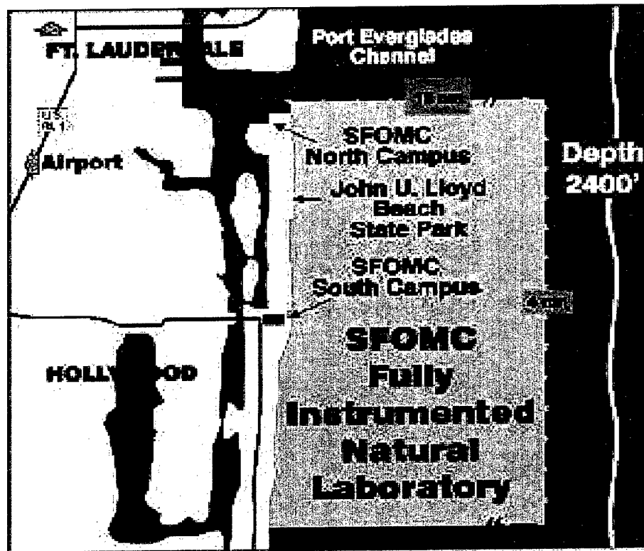
Figure 2.2.1 South Florida Ocean Measurement Center Site
