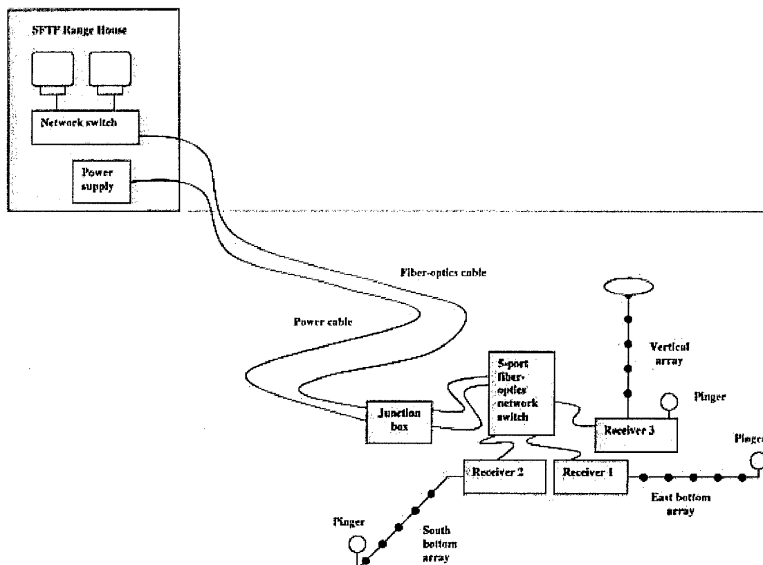
Figure 3.5.12 University of Miami Acoustic Arrays at South Florida Ocean Measurements Center.
