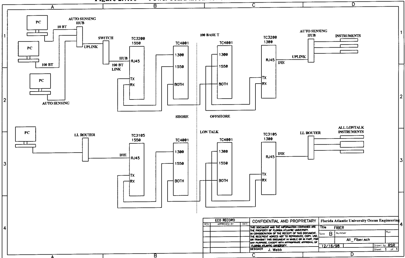
Figure 2.7.11 Fiber-optic Ethernet transceiver connection
