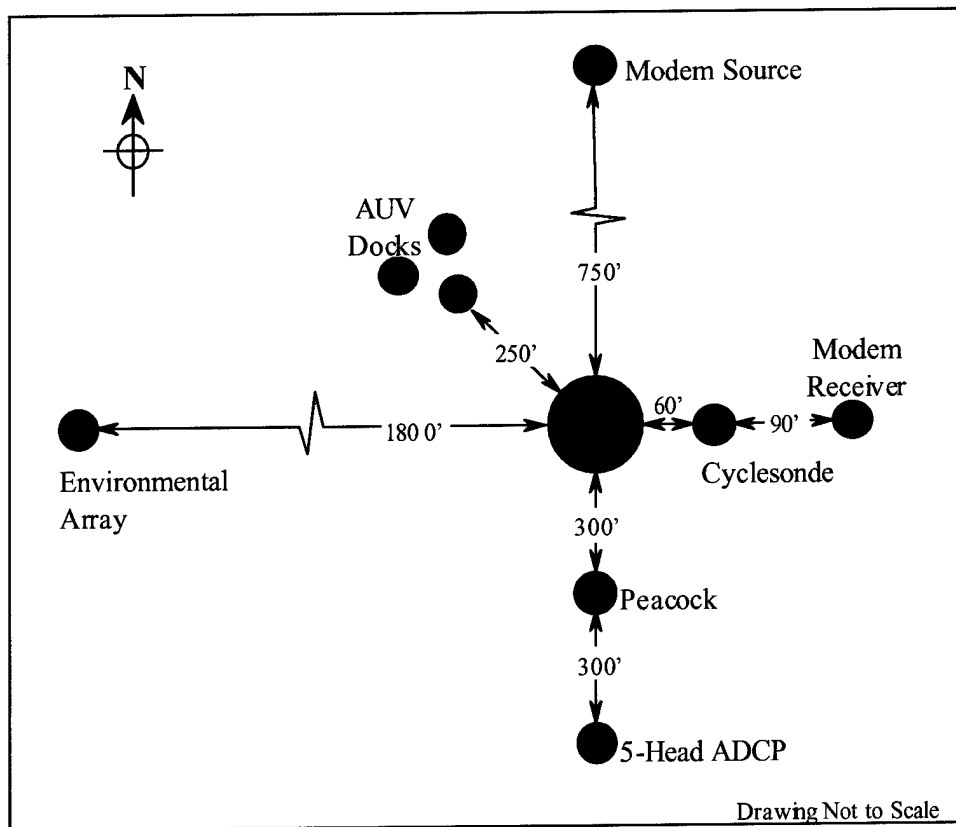
Figure 2.7.2 Instruments co-ordinates relative to the MUX
