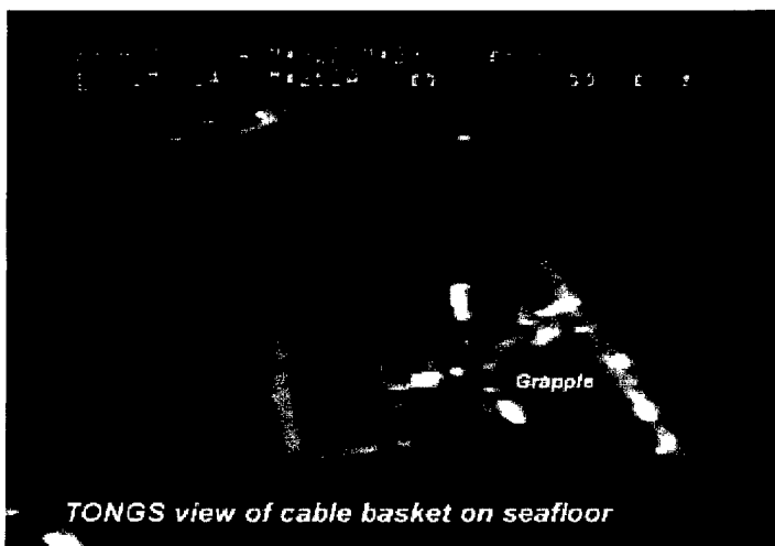
Figure 2.6.4- Picture from TONGS camera as it approaches one of the cable baskets (upper left) to pull out the jumper cable for vertical array. Note the empty basket on the left (used for east bottom array) and the partially full basket on right (used for south array).
