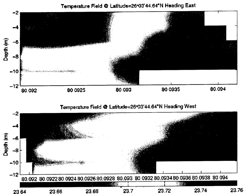
Figure 3.2.1.11. Temperature field, consistent in each direction.
