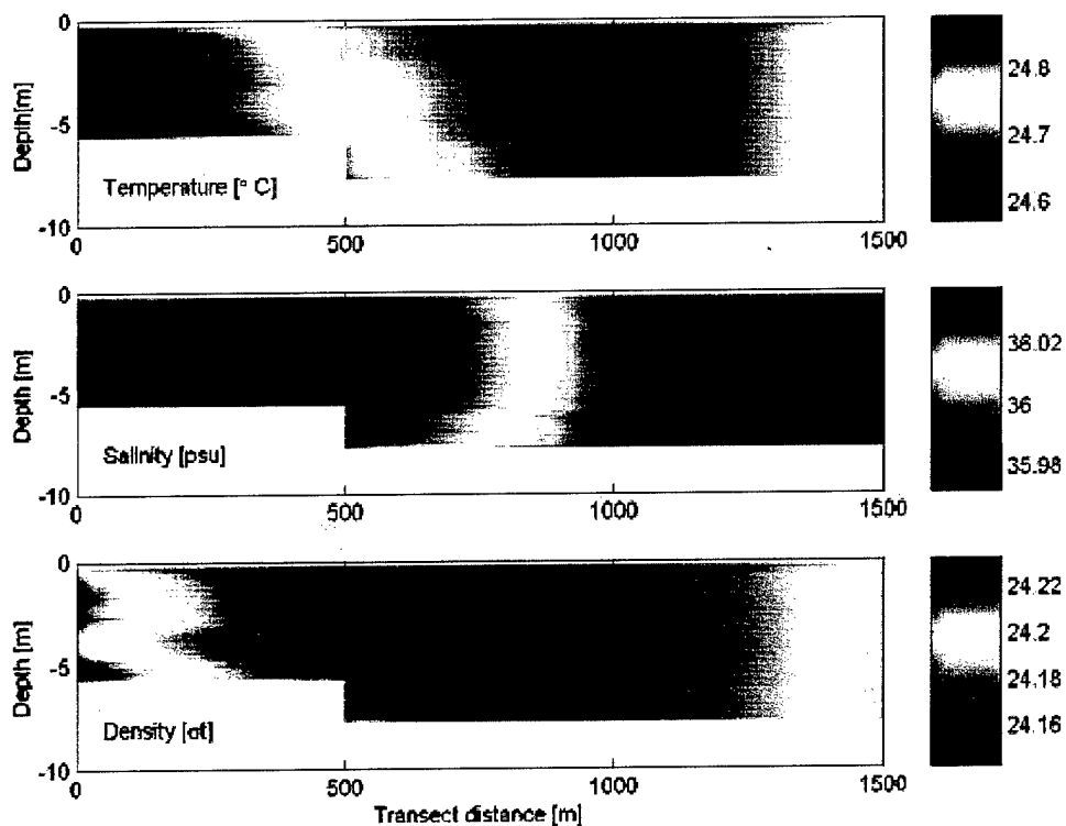
Figure 3.2.1.5d. Composite views of temperature, salinity and density during Dec. 17 over a transect along 26^{\circ} 3.8' N starting at 26^{\circ} 3.8'N 80^{\circ} 5.68'W .
