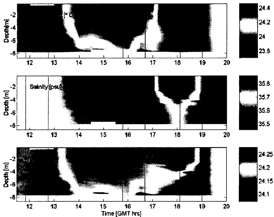
Figure 3.2.1.5a. Composite views of temperature, salinity and density during Dec. 17 at 26^{\circ} 3.83'N 80^{\circ} 5.68'W .
