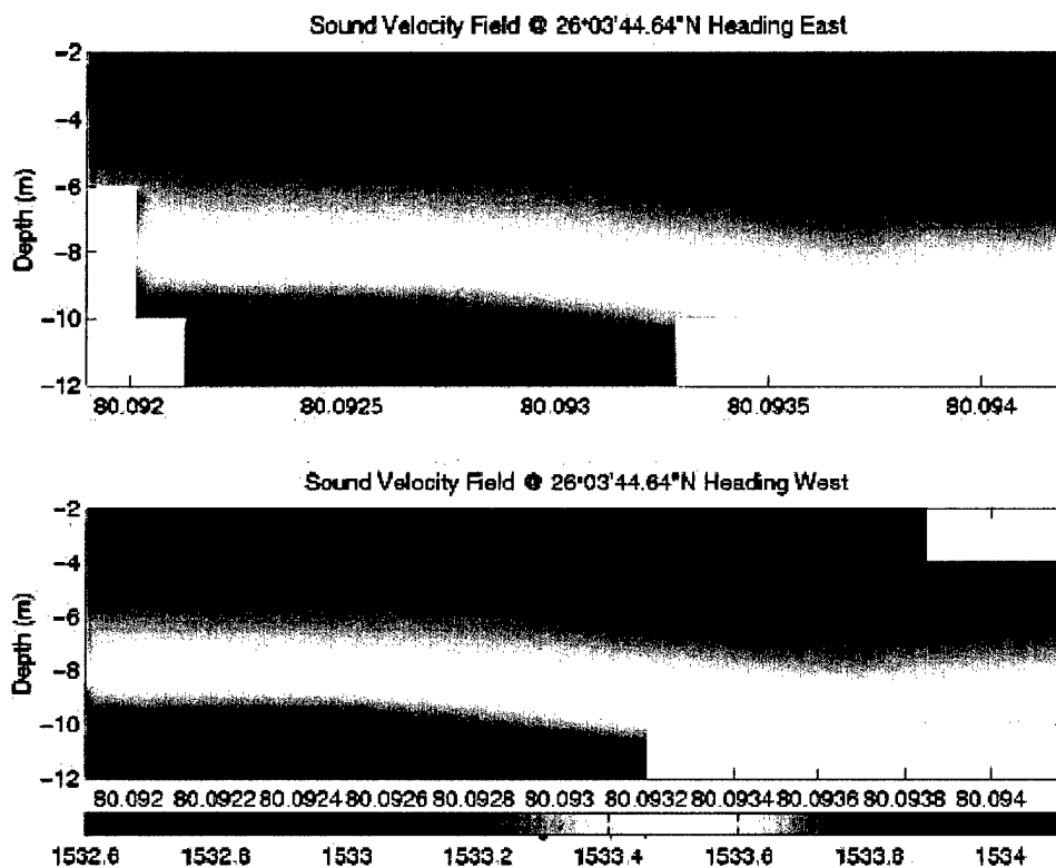
Figure 3.2.1.13. Sample speed of sound; it appears to be mainly a function of depth, since variations in salinity and temperature are small.
