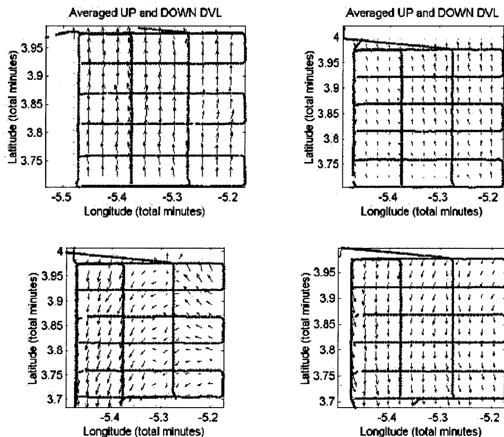
Figure 3.3.7: Four maps of the depth-averaged current vectors acquired from the ADCPs on the AUV during the 4D01a mission a) 0-1.5 h, b) 1.5-3 h, c) 3-4.5 h, and d) 4.5-6 h. Each map represents one realization over about 1.5 h to complete the lawn-mower pattern (AUV-tracks are solid) over a 500 m x 500 m grid.
