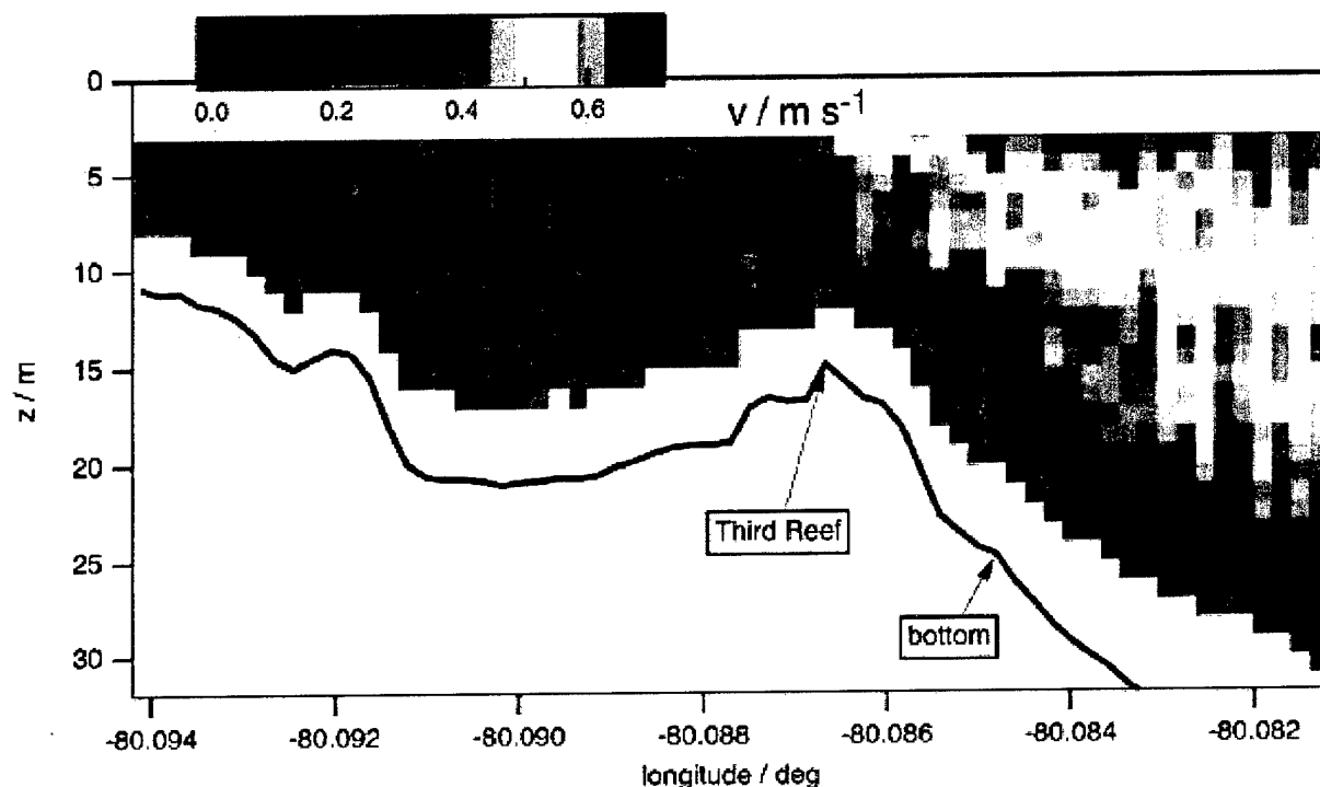
Figure 3.3.4: Cross-shelf section of the along-shelf current observed from the 600kHz ADCP on the R/V Stephan on 1704-1719 GMT 9 July 99. Northward current prevailed over this section with maximum currents near to the surface.
