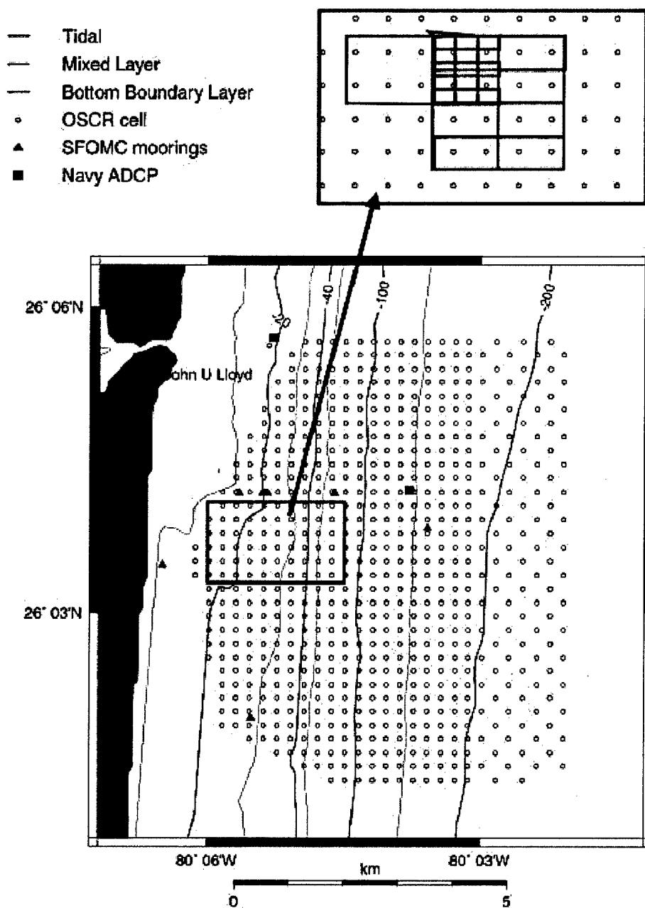
Figure 3.3.1. Multiple-nested measurement domain embedded with the OSCAR grid (circles) for the SFOMC 4-D Current Experiment relative to bottom topography in meters. Master and slave sites are located at John Lloyd State Park and Hollywood Beach, respectively. Inset provide the high-resolution sampling patterns for AUV measurements relative to OSCAR Cells for the Mixed Layer, Bottom Boundary Layer, and Tidal Missions described in Table 3.3.1. The ship track was located 1-2 OSCAR cells removed from the AUV-missions.
