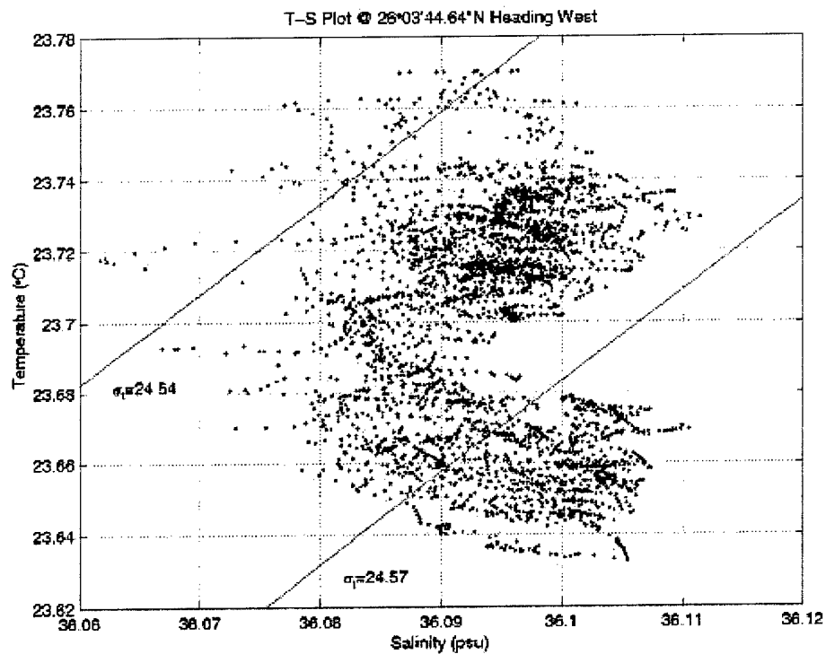
Figure 3.2.1.14. T-S plots early morning on 12/17/99. Note range for comparison to later date.
