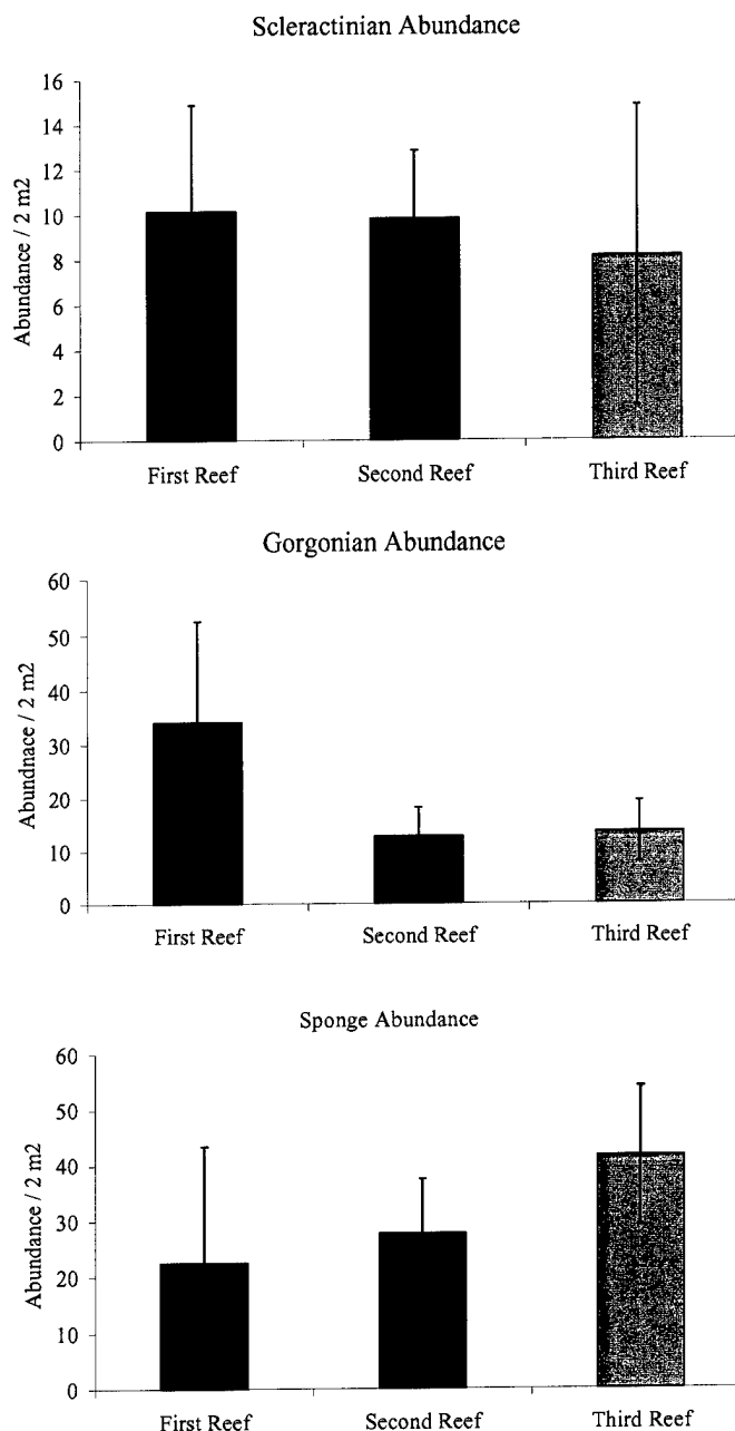
Figure 3.6.3.1: Scleractinian, gorgonian, and sponge abundance (mean \pm 1 SE) for each of the three reefs within the range.
