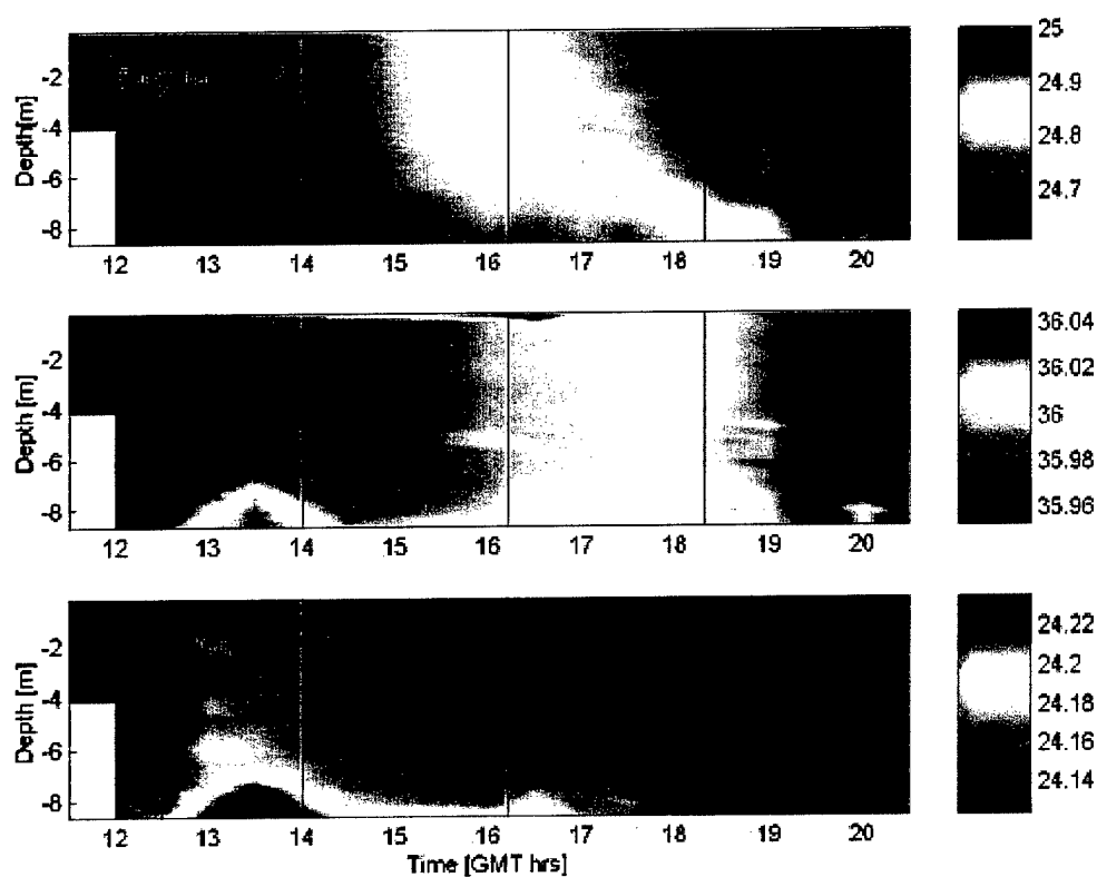
Figure 3.2.1.5c. Composite views of temperature, salinity and density during Dec. 21 at 26^{\circ} 3.83'N 80^{\circ} 5.68'W .
