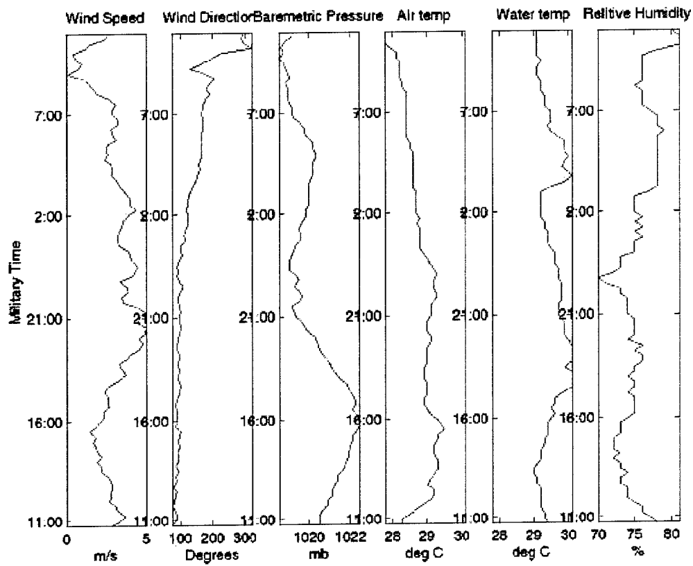
Figure 3.2.2.8: Weather data corresponding to the 27hr mission started on 07/22/99
