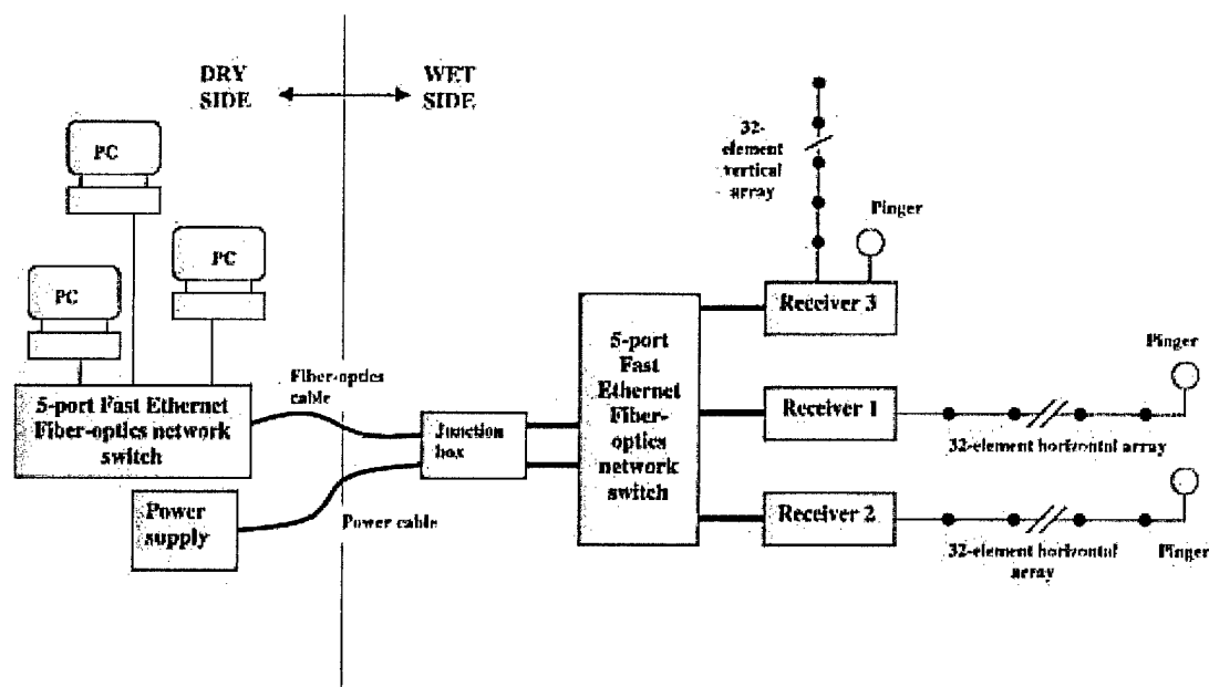
Figure 3.5.9. System block diagram
