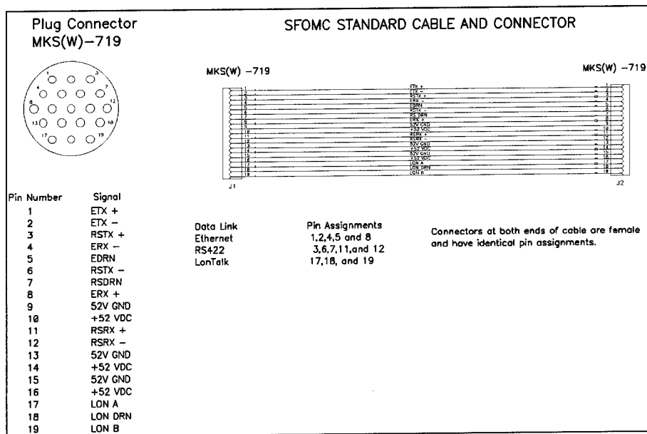
Figure 2.7.6 Generic instrument cable/connector pinouts
