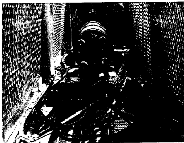
Figure 3.5.14 The Multiplexer Pressure Housing
