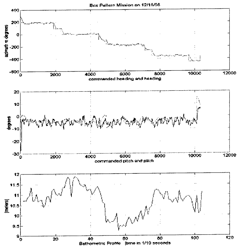
Figure 3.2.1.16. MADD OG AUV data, illustrating its performance.
