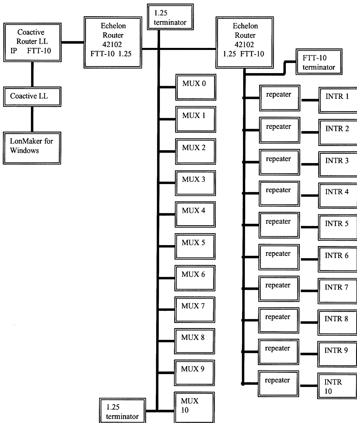
Figure 2.7.12 A block diagram of LonTalk connection
