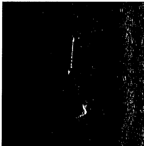
Figure 3.1.6: Mission 19981211.1630. (a) Plot of vehicles path. Starting point is at origin. The AUV transited to the survey site and then surveyed the two lines of mines with a 3 meter spacing between each path. (b) Blow up of a side scan image showing torpedo and concrete block.
