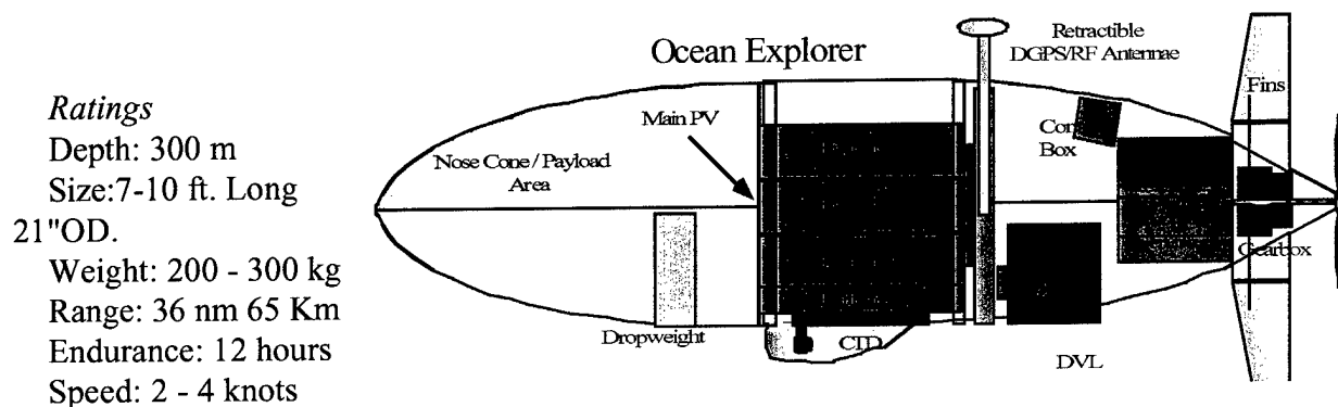
Figure 3.1.1 Ocean Explorer Autonomous Underwater Vehicle base configuration
