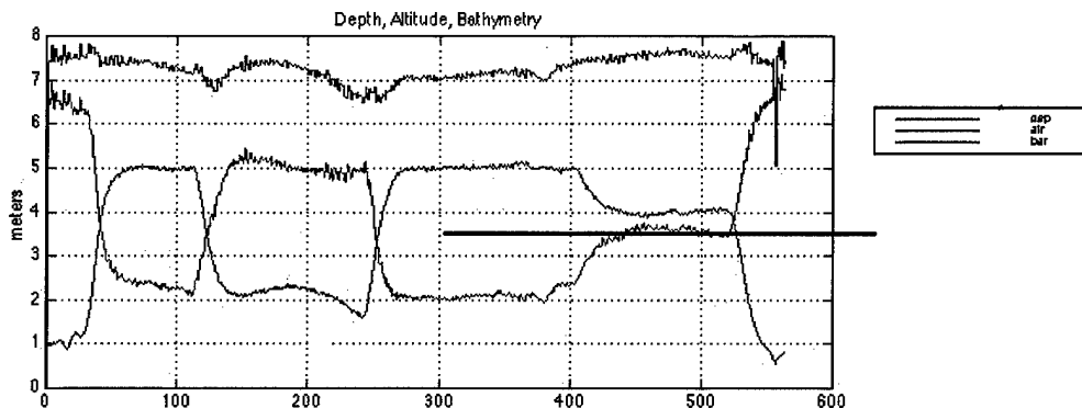
Figure 3.2.3.6 : Depth Performance
