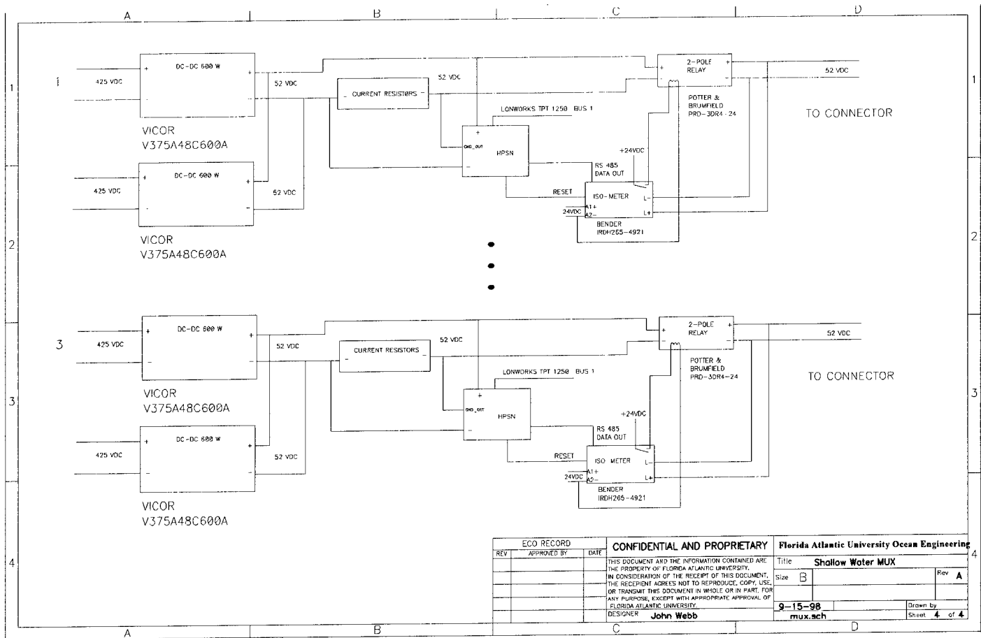
Figure 2.7.10 Power board layout for one of the AUV docks
